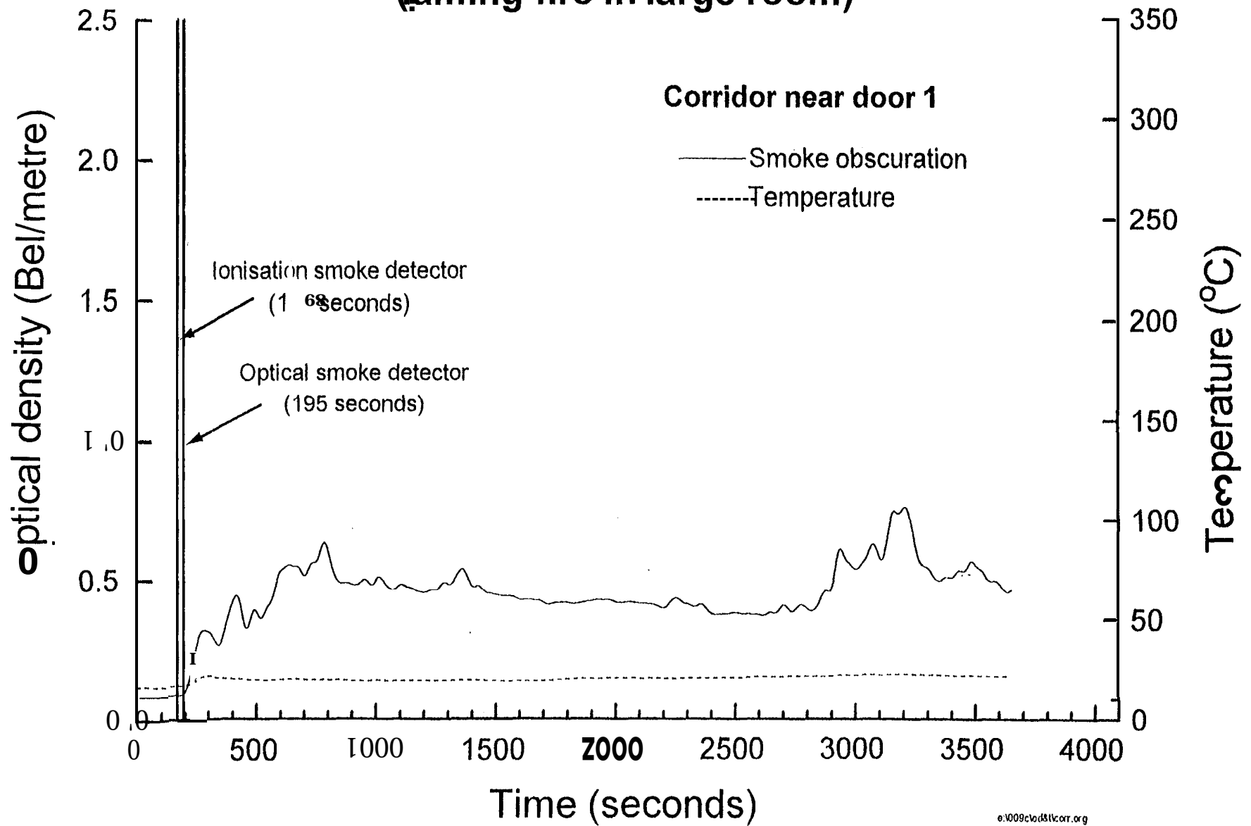
Fig. 8.2.8-1 Smoke obscuration - Test FML1 (flaming fire in large room)
