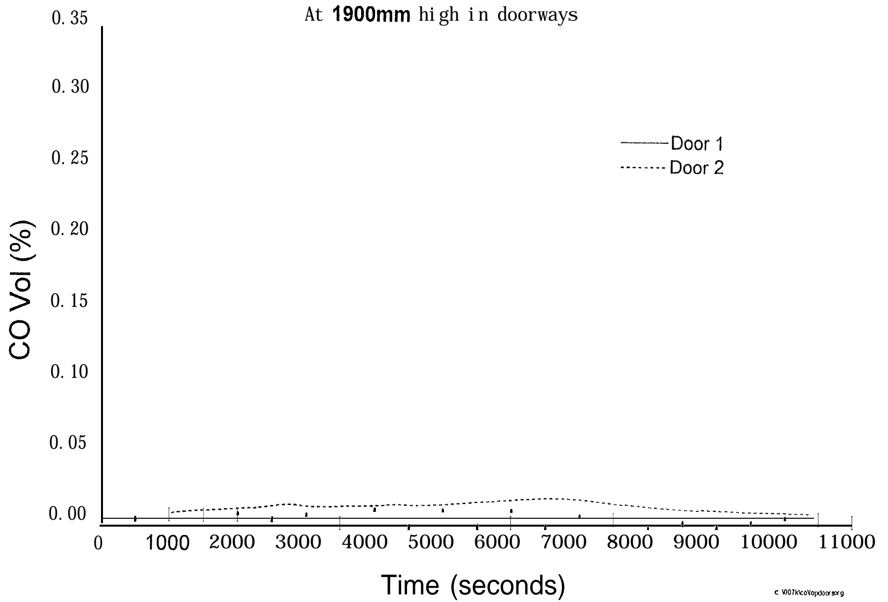
Fig. 6.2.3-8 Carbon monoxide concentration (Smouldering) - Test SM8
