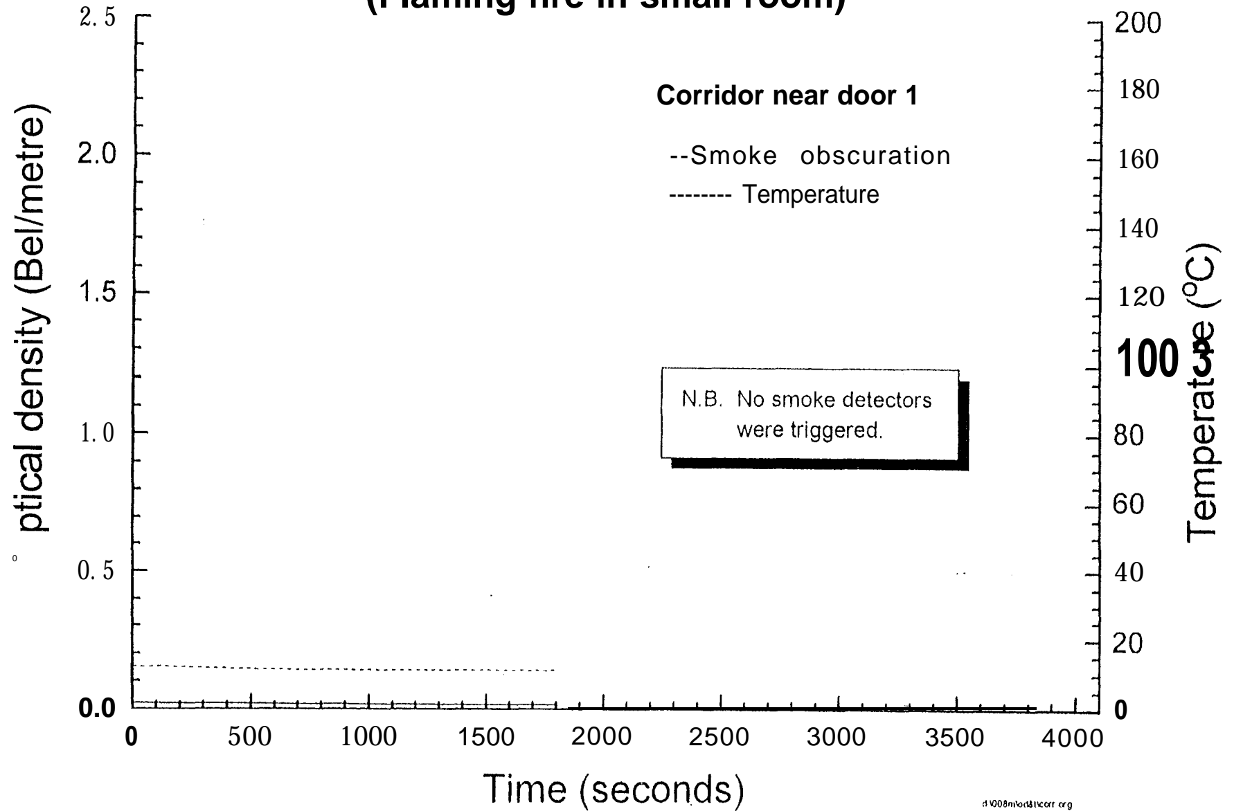
Fig. 7.3.7-10 Smoke obscuration and temperature - Test FMS7 (Flaming fire in small room)
