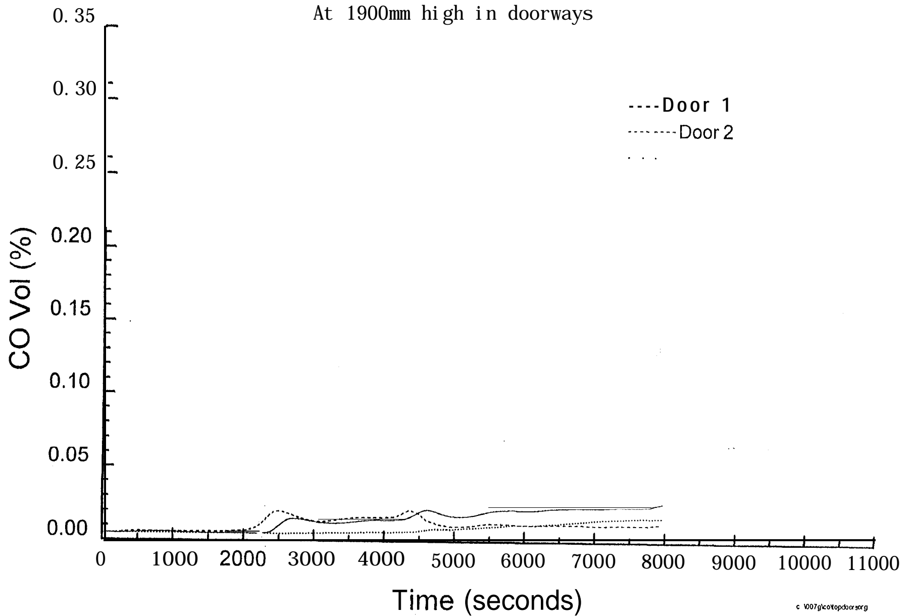
Fig. 6.2.3-5 Carbon monoxide concentration (Smouldering) - Test SM5
