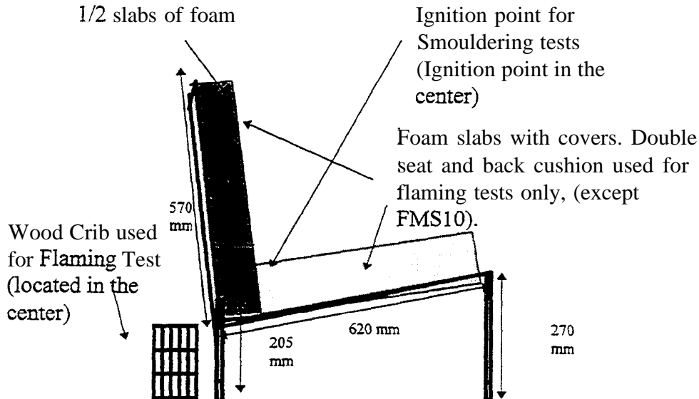
Figure 5-1 Chair Fuel Load for Smouldering and Small Room Flaming Experiments
