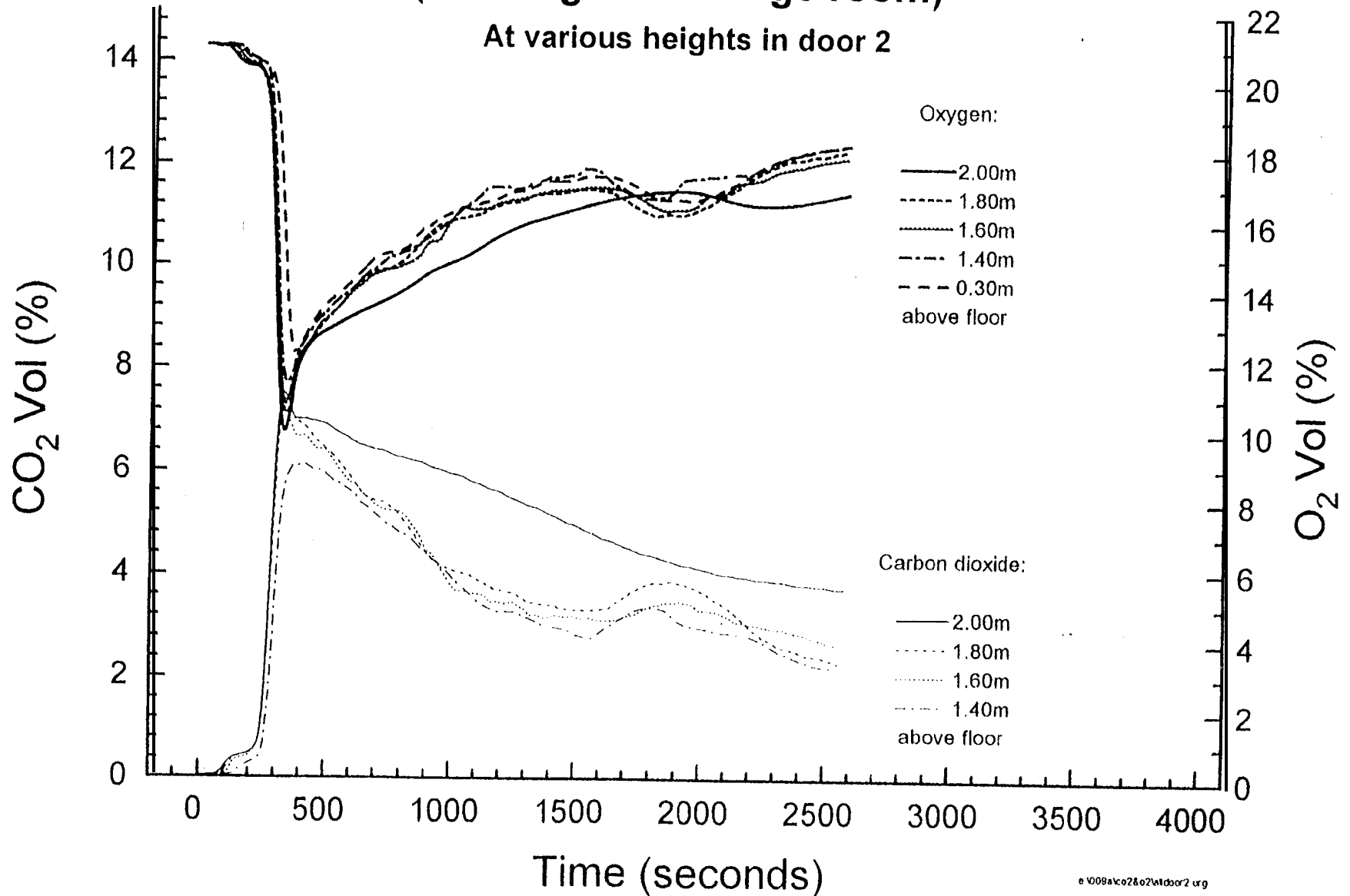
Fig. 8.2.7-10 Carbon dioxide and Oxygen concentrations - Test FML3 (Flaming fire in large room)
