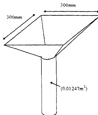
Figure 1 Flowhood construction
