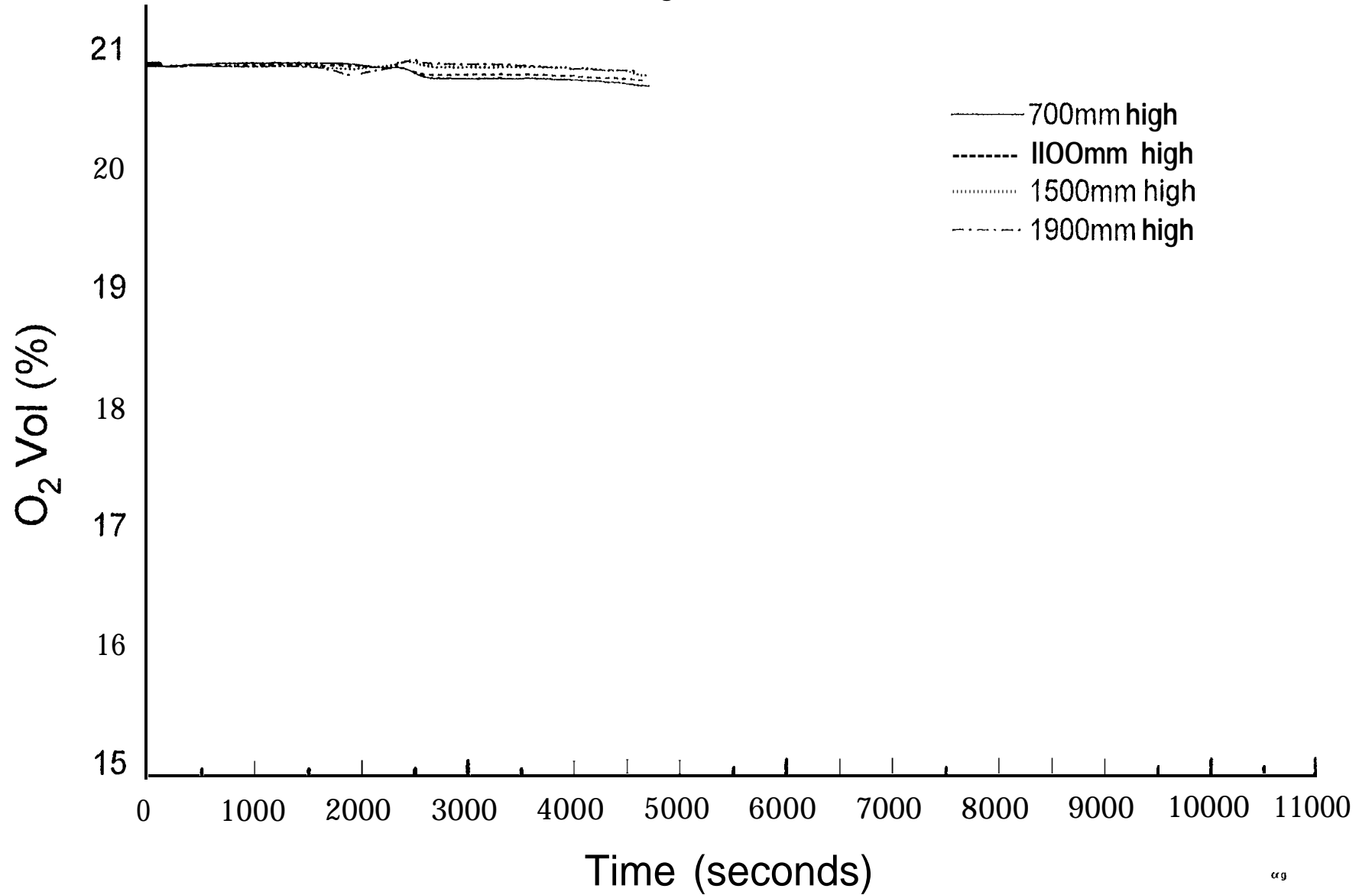
Fig. 6.2.4-3 Oxygen concentration (Smouldering) - Test SM3
