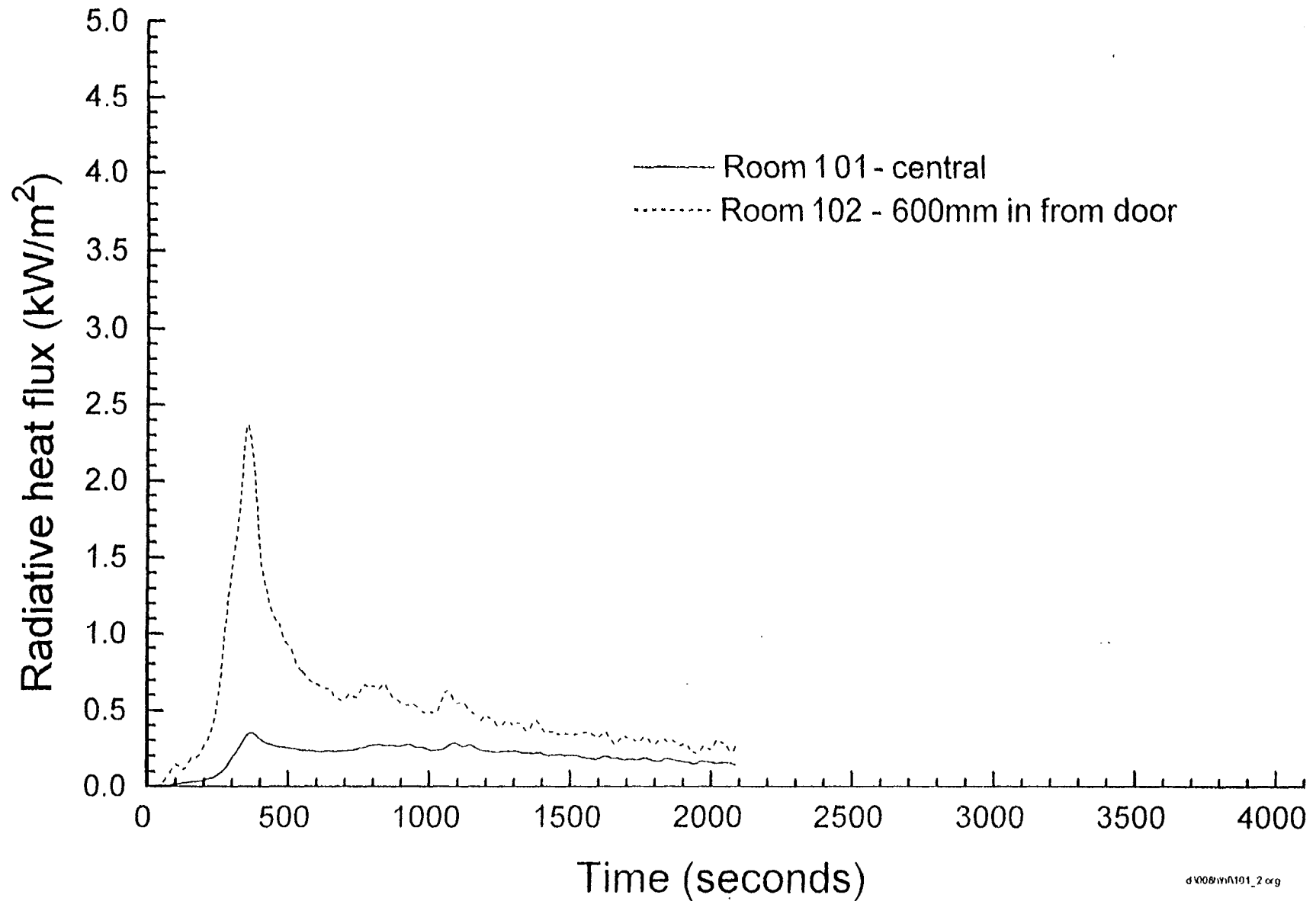
Fig. 7.3.4-5 flux (Flaming fire in small room) - Test FMS8
