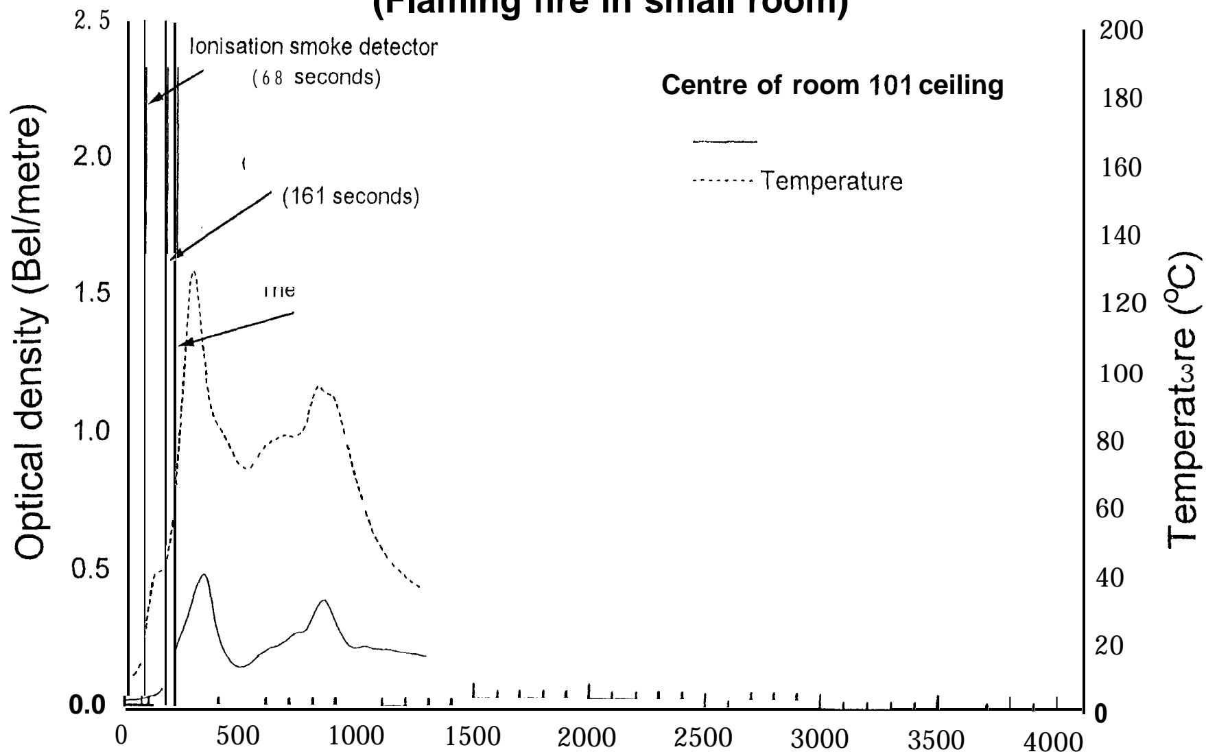
Fig. 7.3.7-6 Smoke obscuration and temperature - Test FMS10 (Flaming fire in small room)
