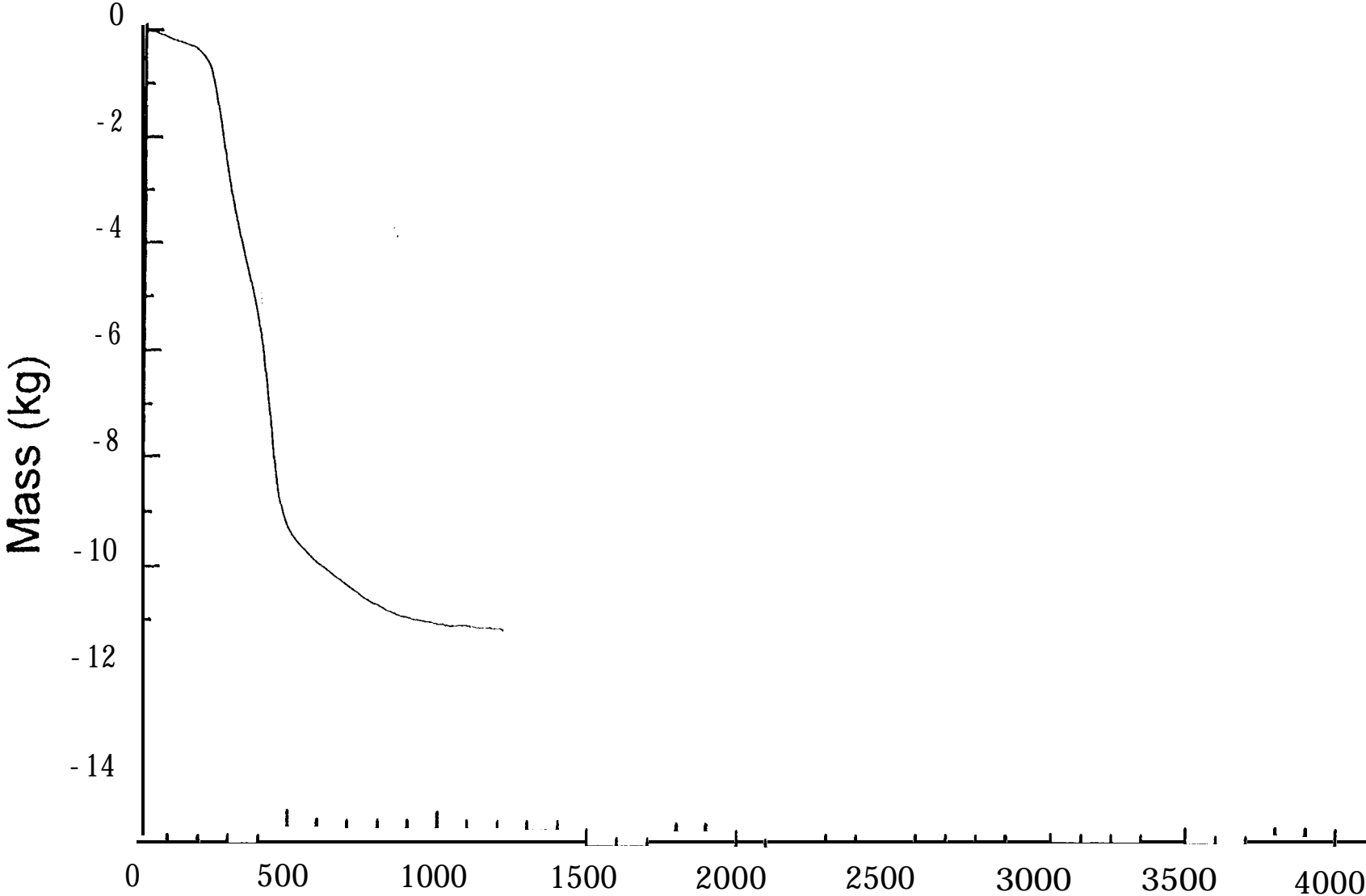
Fig. 8.2.1-5 Mass loss (Flaming fire in large room) - Test FML5
