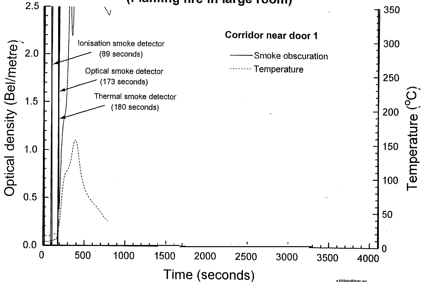
Fig. 8.2.8-6 Smoke obscuration and temperature - Test FML6 (Flaming fire in large room)
