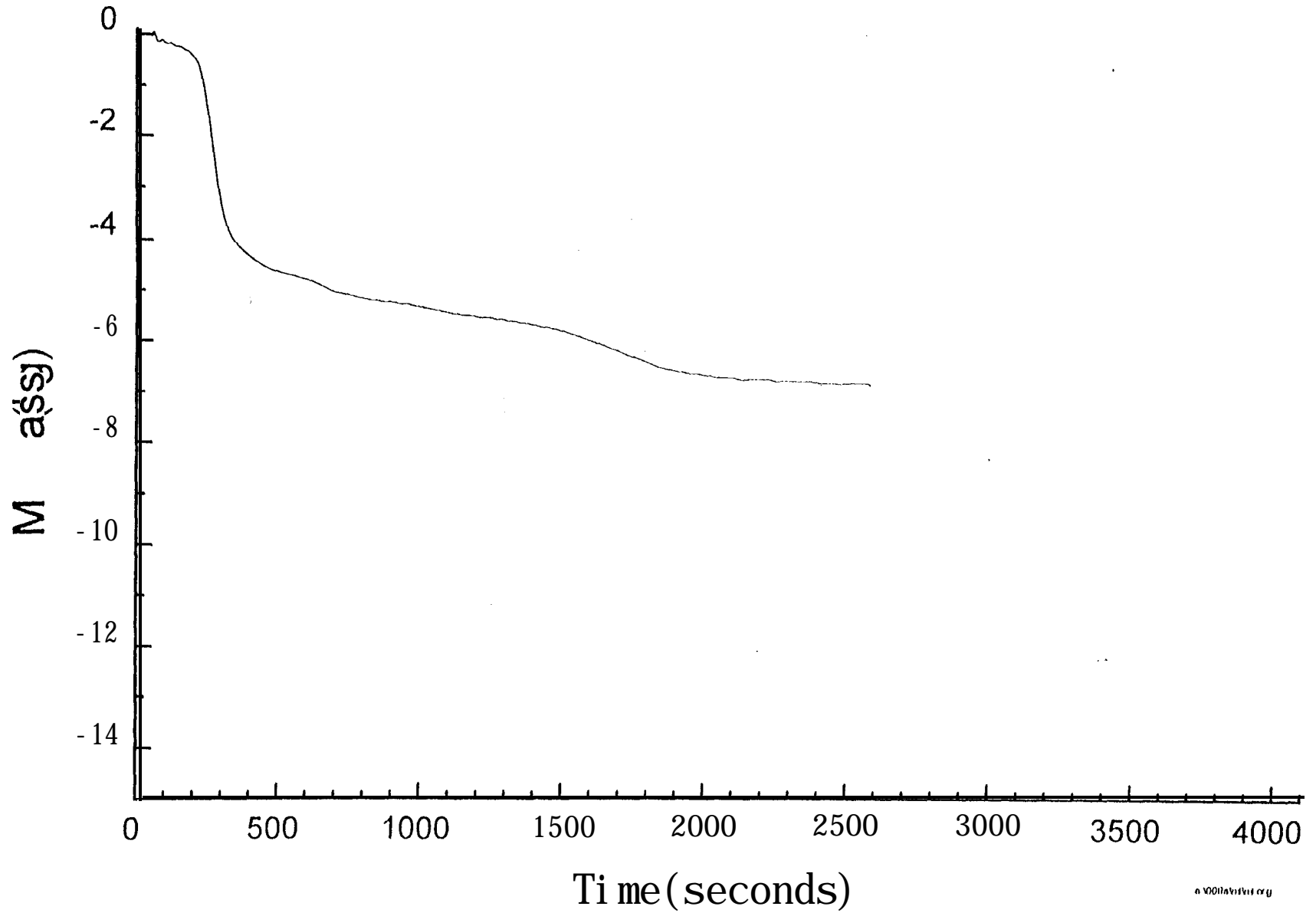
Mass loss (Flaming fire in large room) - Test FML3
