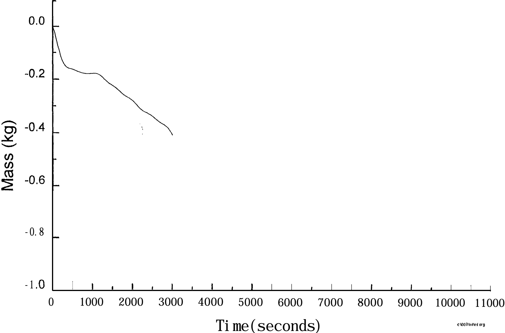
Fig. 6.2.1-4 Mass loss (smouldering) - Test SM4
