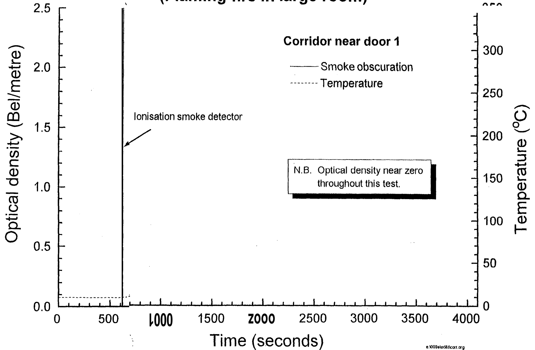
Fig. 8.2.8-2 endtemperature - Test FML2 (Flaming fire in large room)
