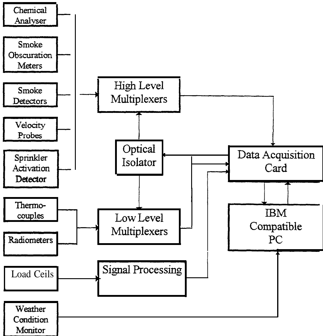
Figure A.15 Data logging system block diagram
