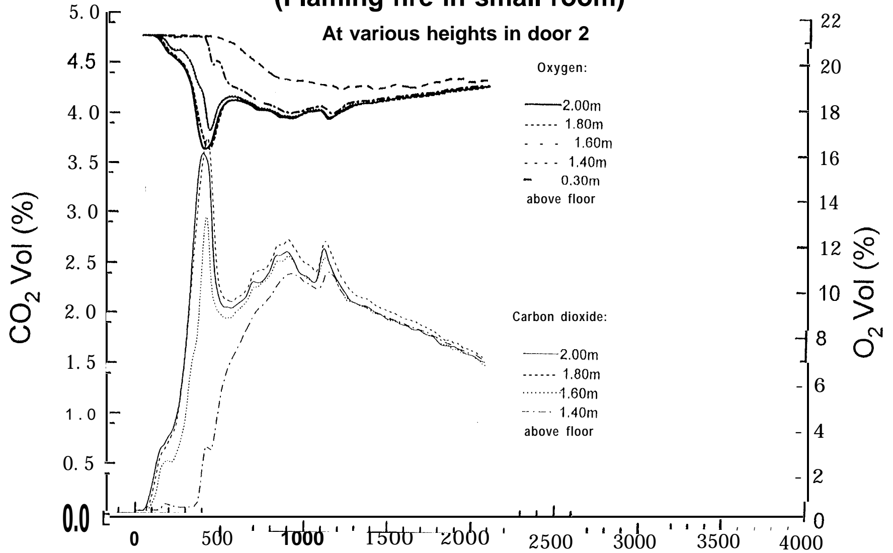
Fig. 7.3.6-I 1 Carbon dioxide and Oxygen concentrations - Test FMS8 (Flaming fire in small room)
