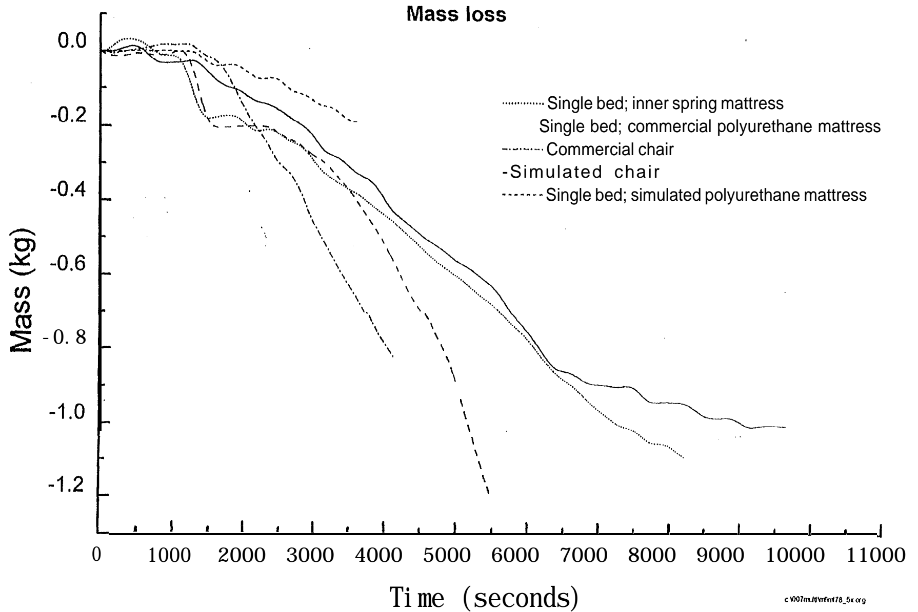
Fig. 6.1 .1-1 Commercial product tests (smouldering)
