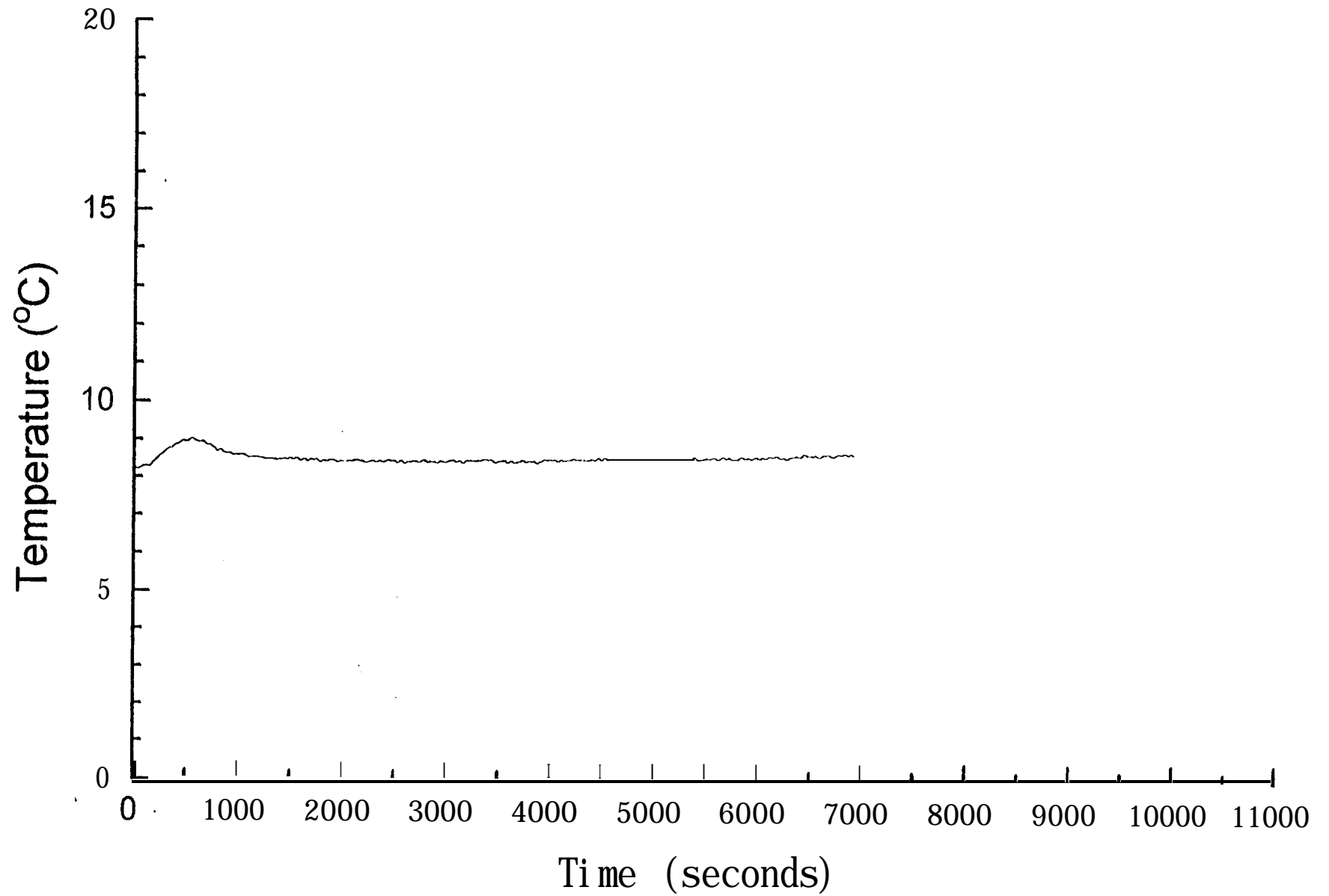
Average temperature in room 101 (Smouldering) - Test SM1
