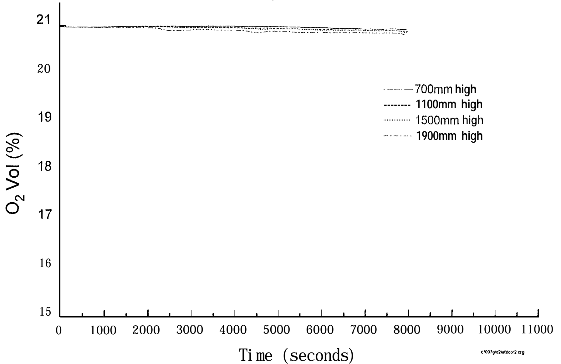
Fig. 6.2.4-5 Oxygen concentration (Smouldering) - Test SM5
