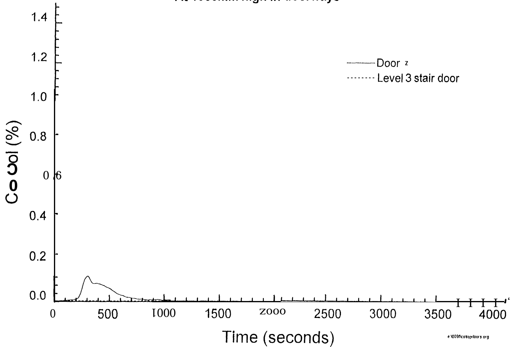
Fig. 8.2.6-4 concentration (Flaming fire in large room) - Test FML4 At 1900mm high in doorways
