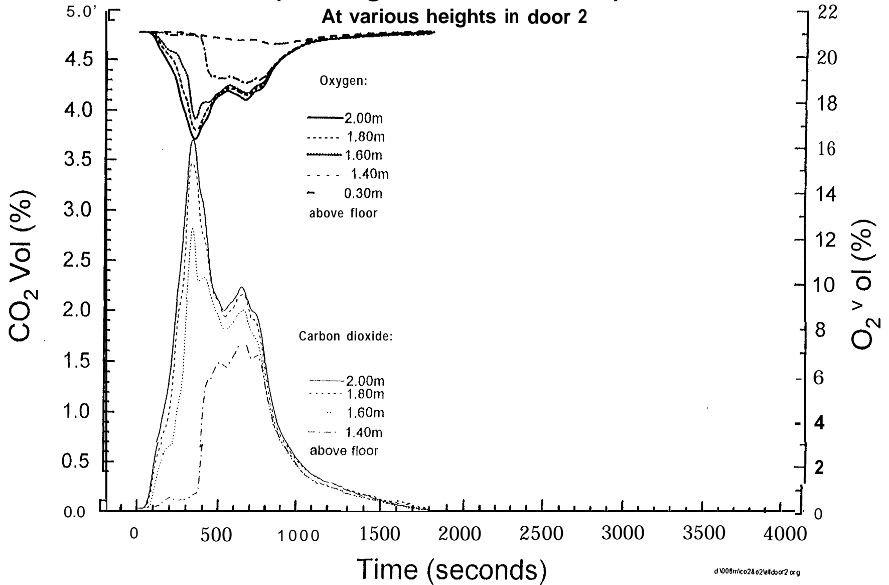
Fig. 7.3.6-I 0 Carbon dioxide and Oxygen concentrations - Test FMS7 (Flaming fire in small room)
