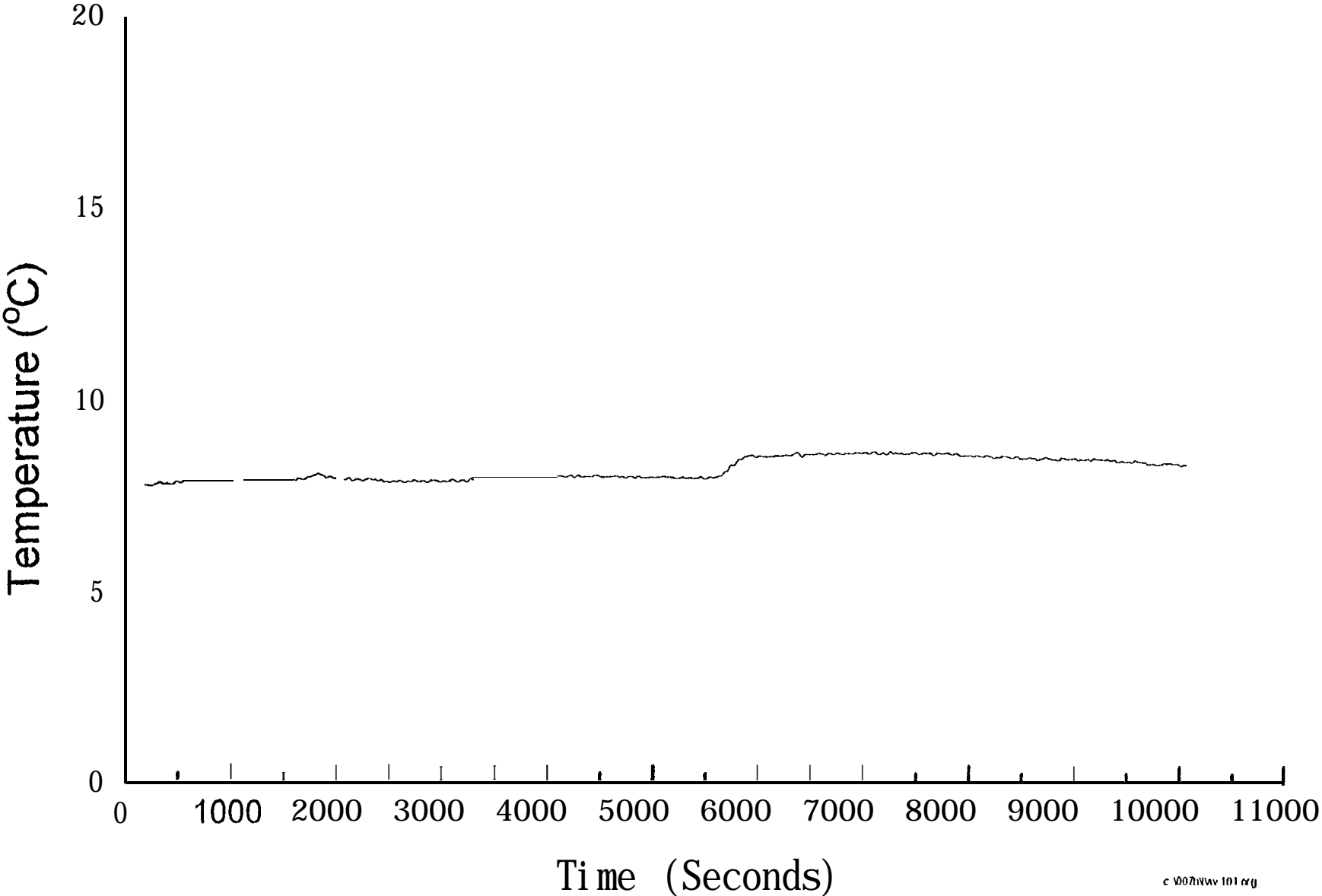
Fig. 6.2.2-I 0 Average temperature in room 101 (Smouldering) - Test SM2
