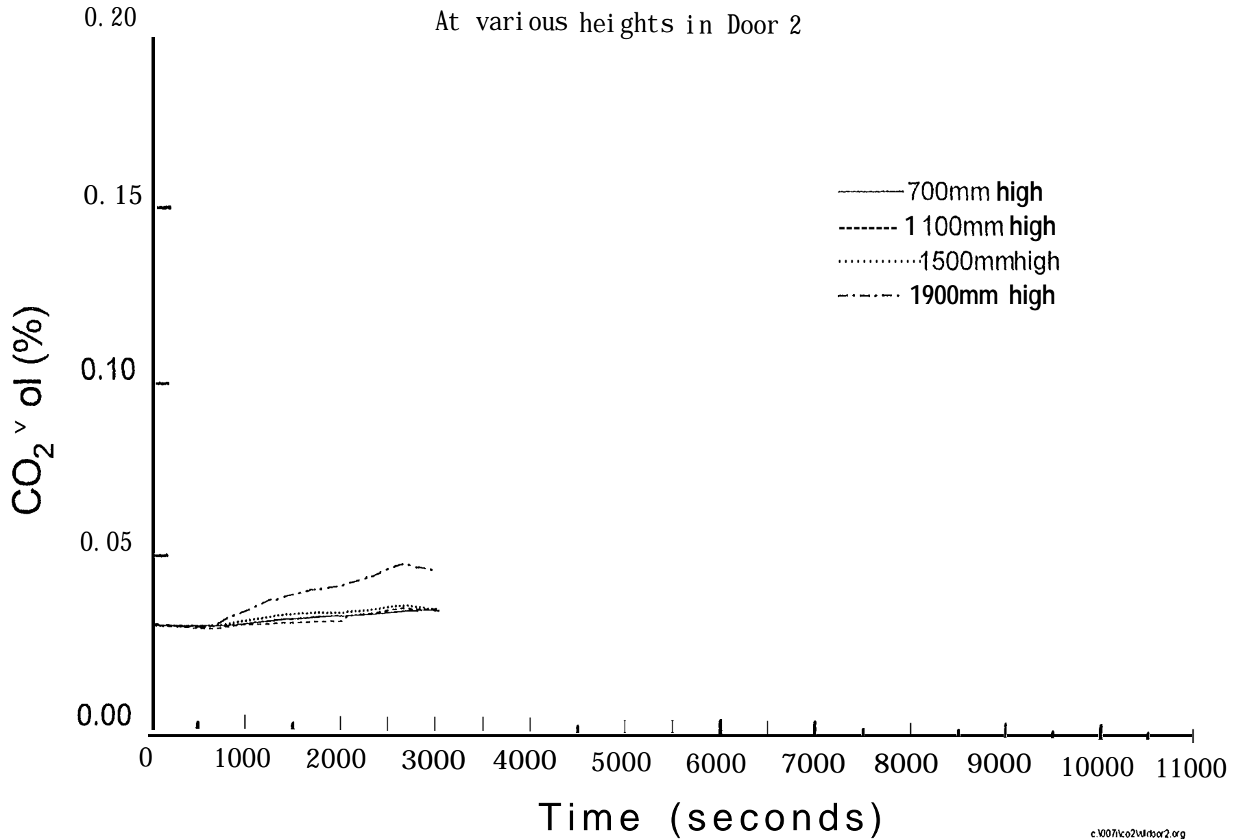
Fig. 6.2.5-3 Carbon dioxide concentration (Smouldering) - Test SM4
