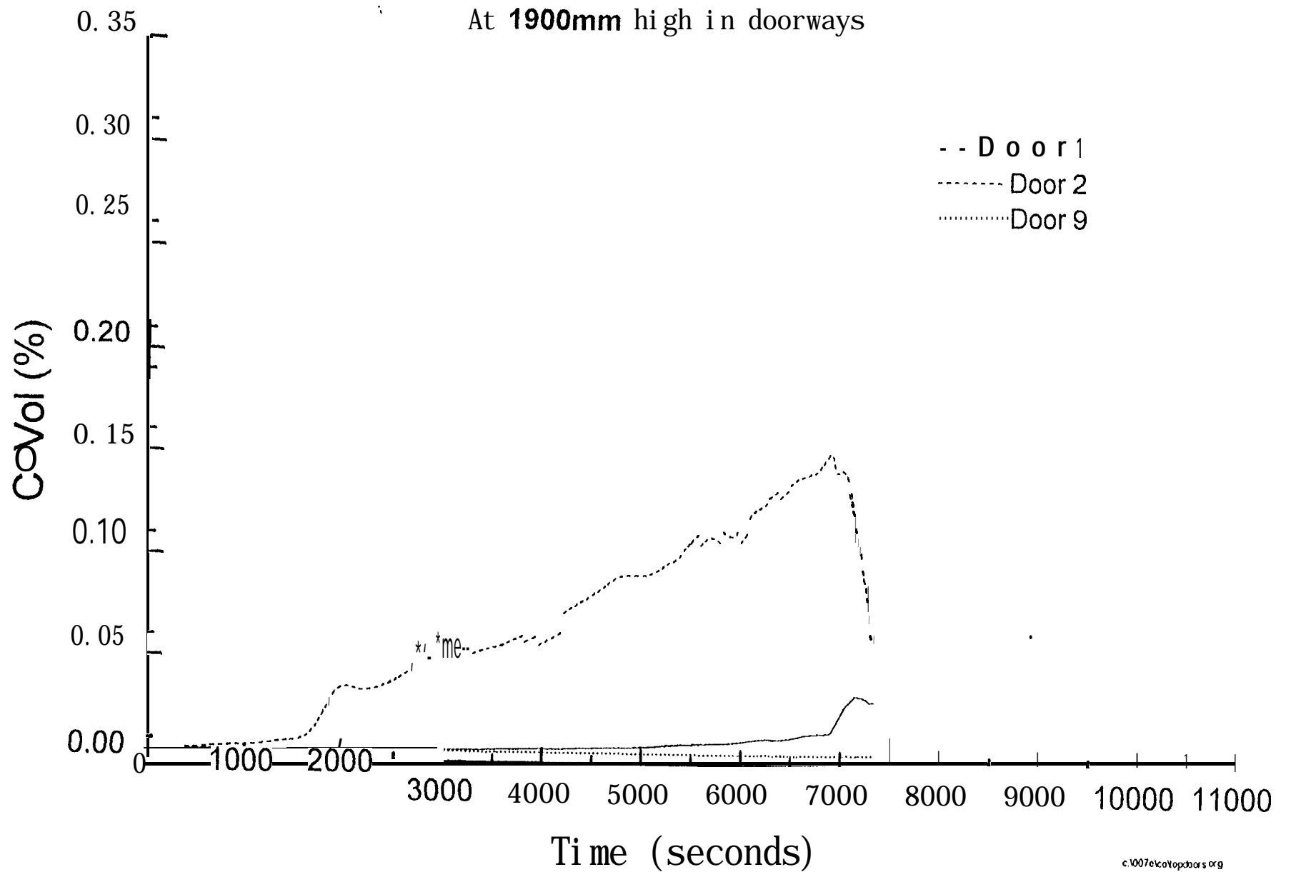
Fig. 6.2.3-1 Carbon monoxide concentration (Smouldering) - Test SM1
