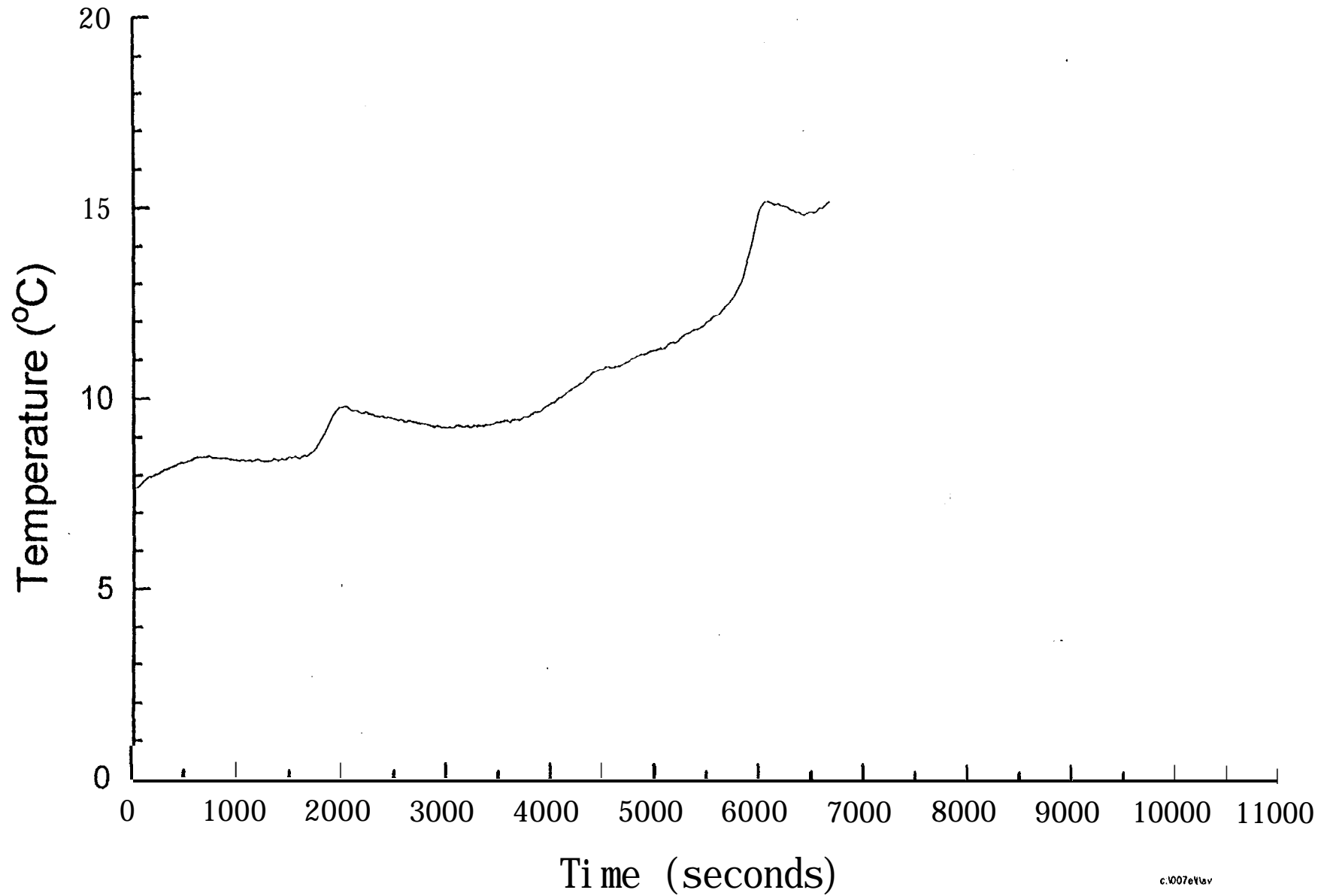
Average temperature in room 102 (Smouldering) - Test SM1
