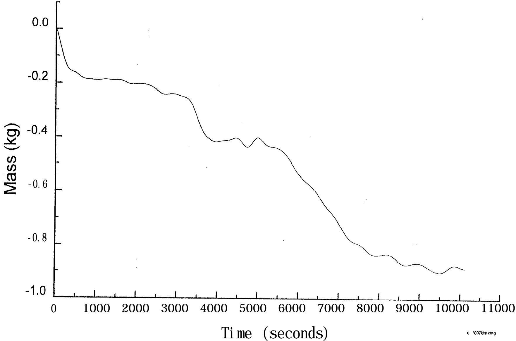
Fig. 6.2.4-8 Mass loss (smouldering) - Test SM8
