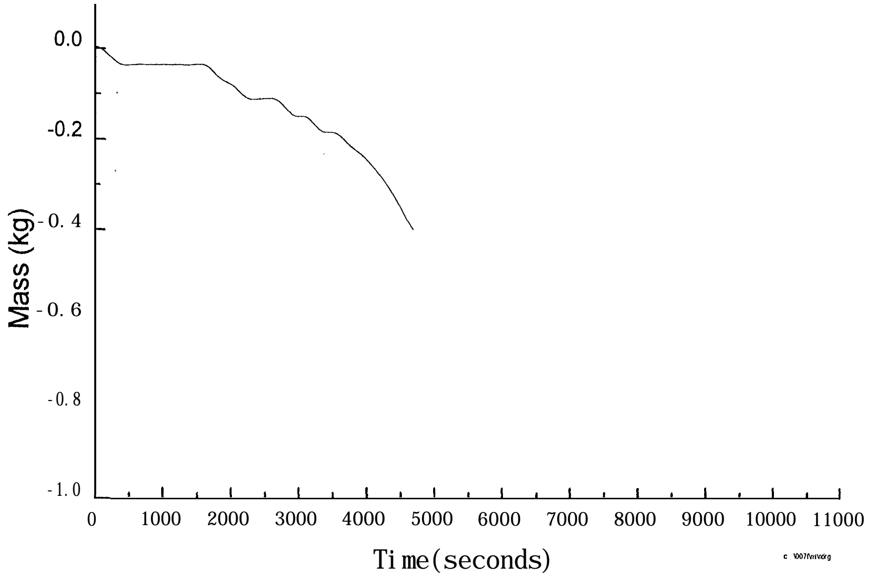
Fig. 6.2.1-3 Mass loss (smouldering) - Test SM3
