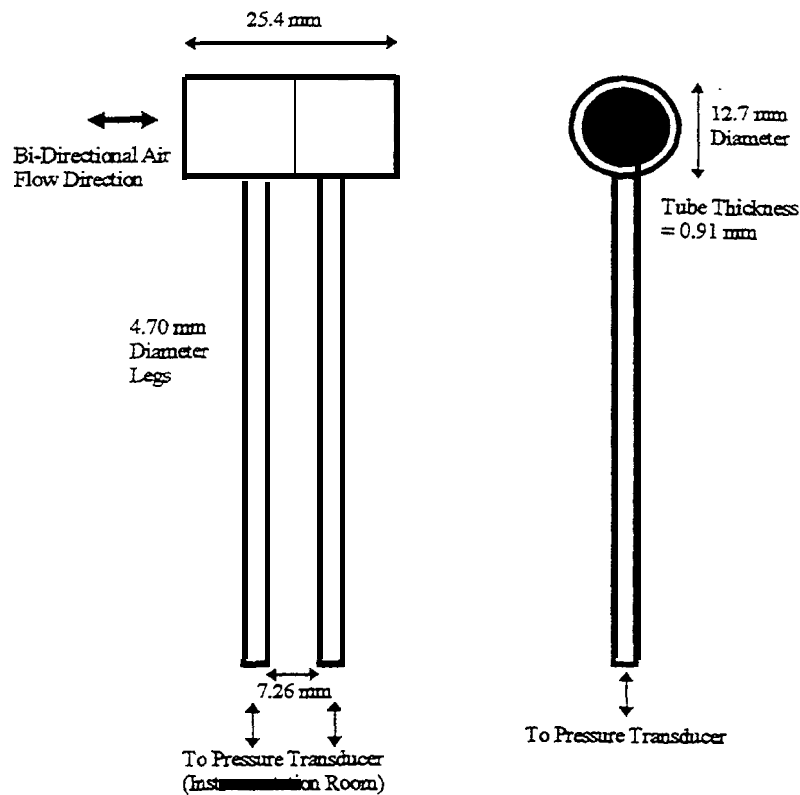
Figure A.12 McCaffrey velocity probe.
