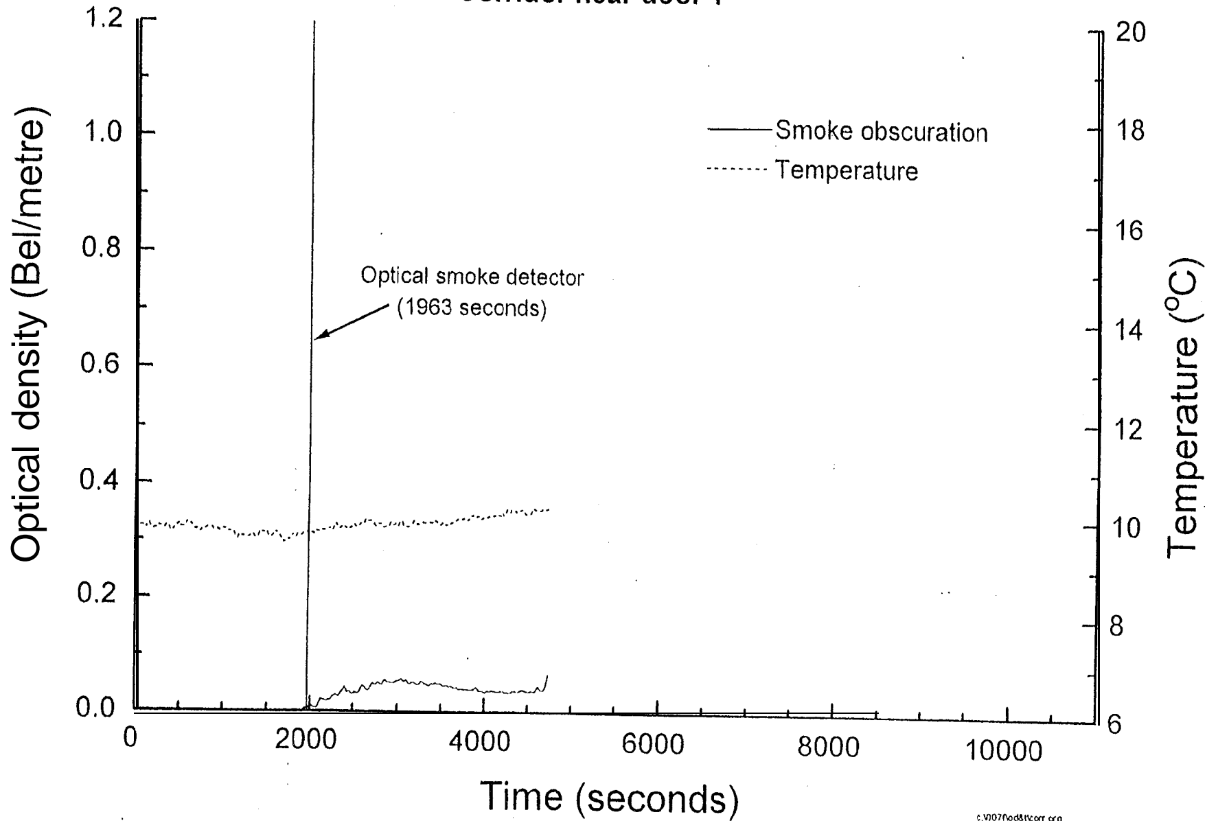
Fig. 6.2.7-11 Smoke obscuration and temperature (smouldering) - Test SM3
