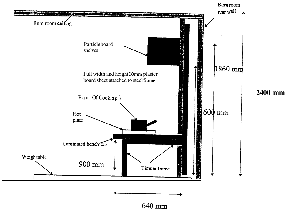
Figure 5-3: Cross section view of Kitchen Mock up used in Small Room Flaming Fire Experiments
