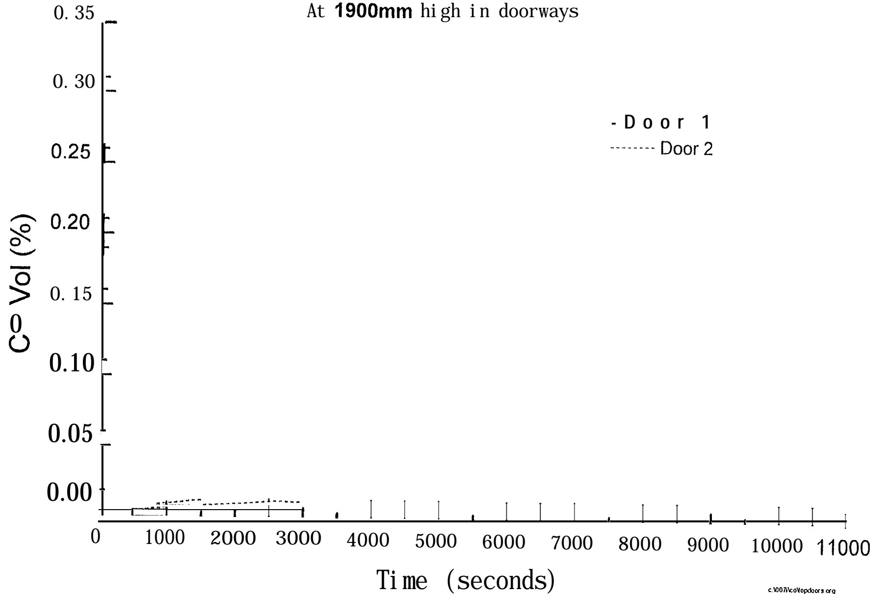
Fig. 6.2.3-4 Carbon monoxide concentration (Smouldering) - Test SM4
