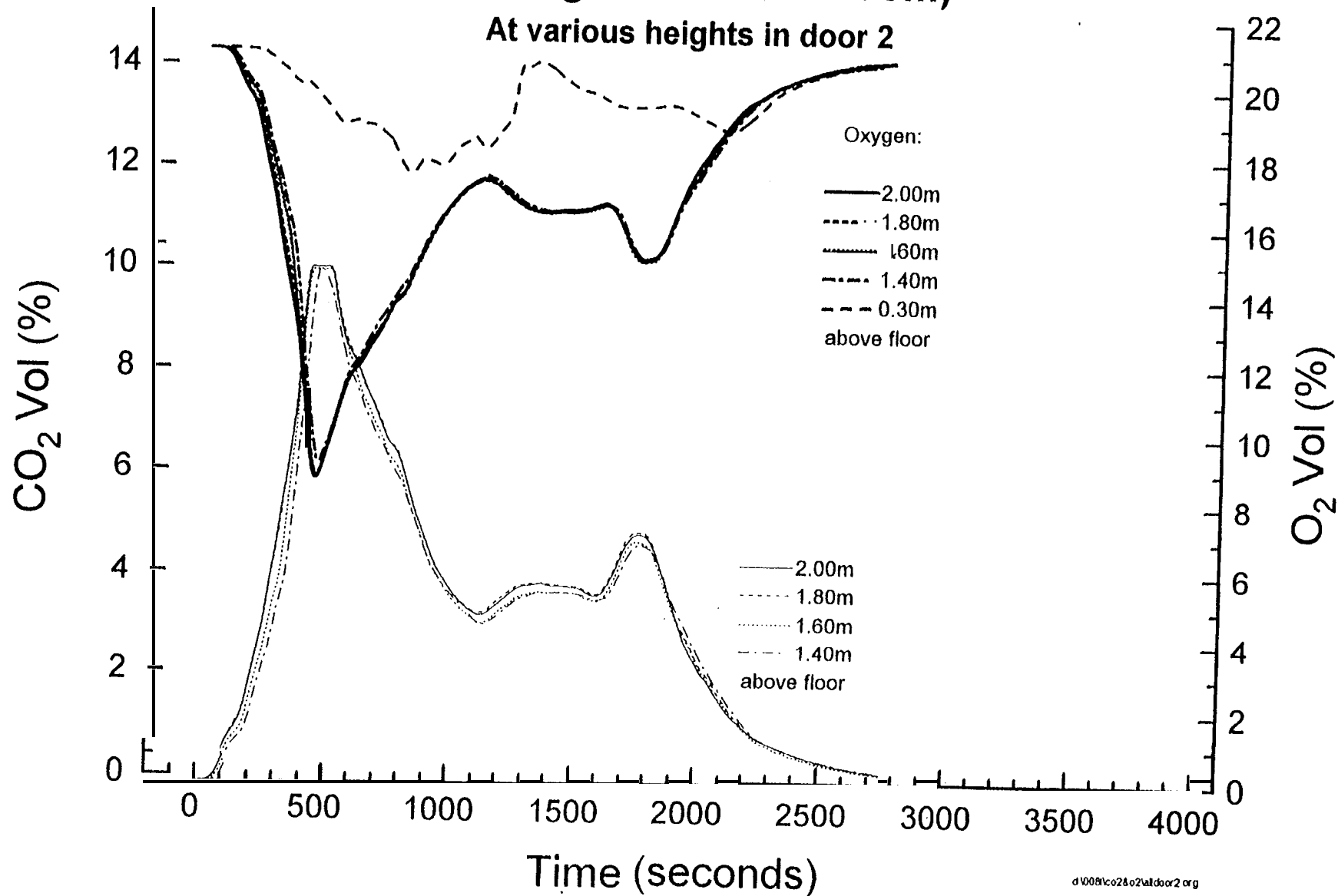
Fig. 7.3.6-8 and Oxygen concentrations - Test FMS5 (Flaming fire in small room)
