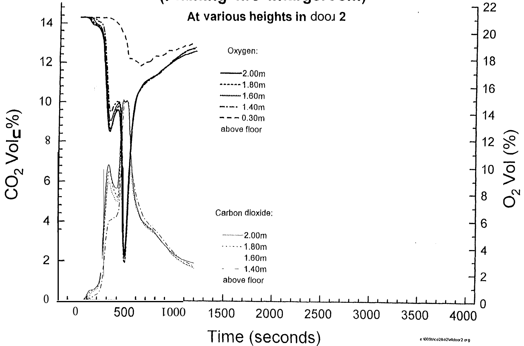
Fig. 8.2.7-1 2 and Oxygen concentrations - Test ML5 (Flaming fire in larger room)
