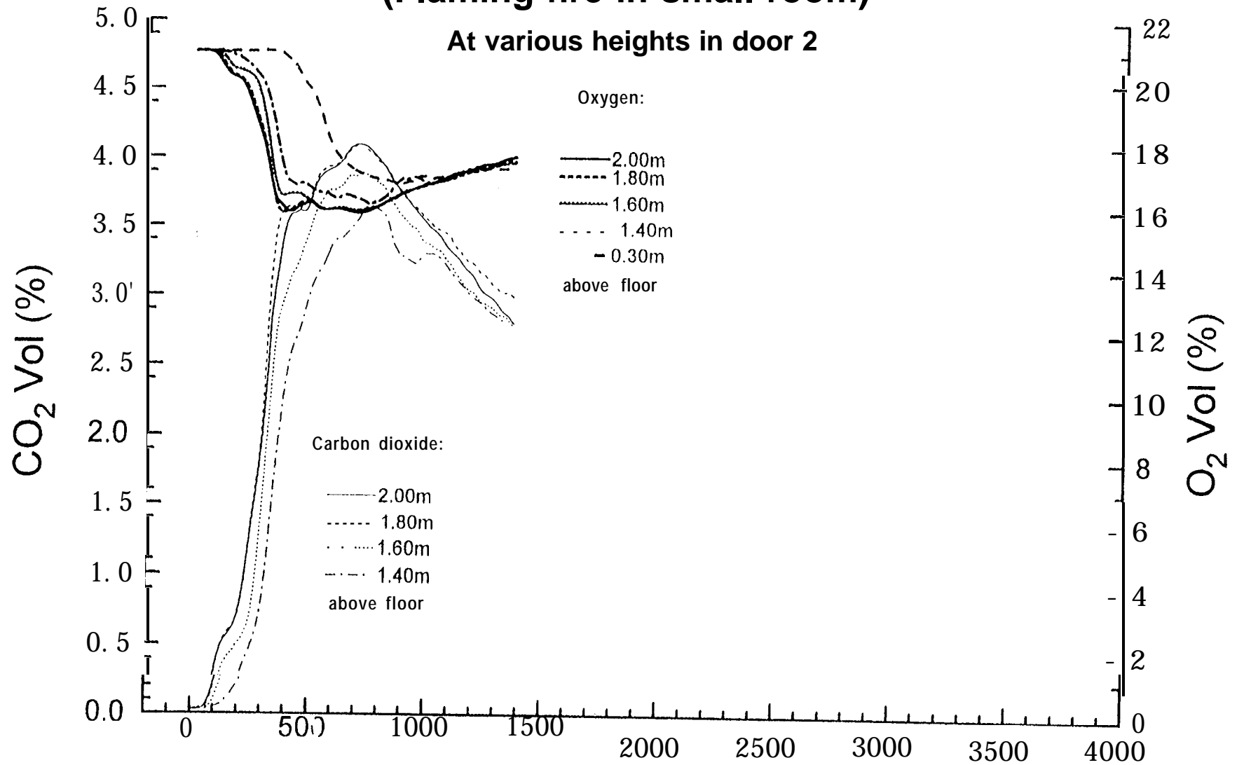
Fig. 7.3.6-9 Carbon dioxide and Oxygen concentrations - Test FMS6 (Flaming fire in small room)
