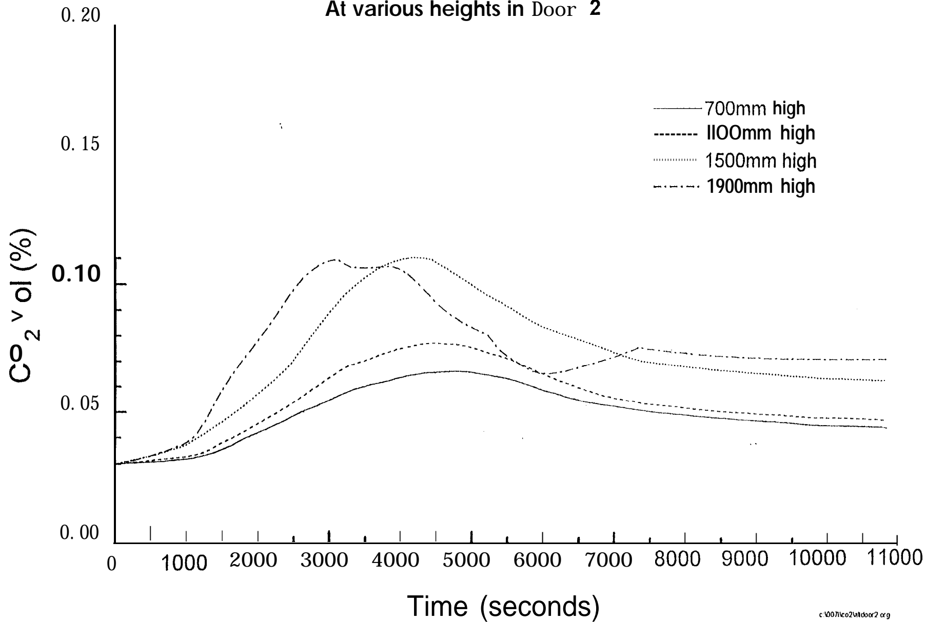
Fig. 6.2.5-6 Carbon dioxide concentration (Smouldering) - Test SM7
