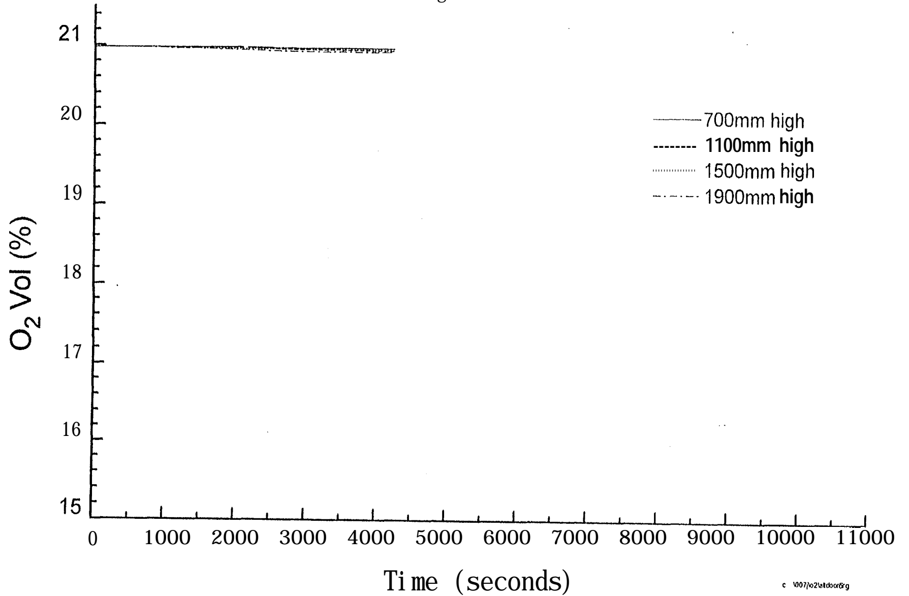
Fig. 6.2.4-6 Oxygen concentration (Smouldering) - Test SM6
