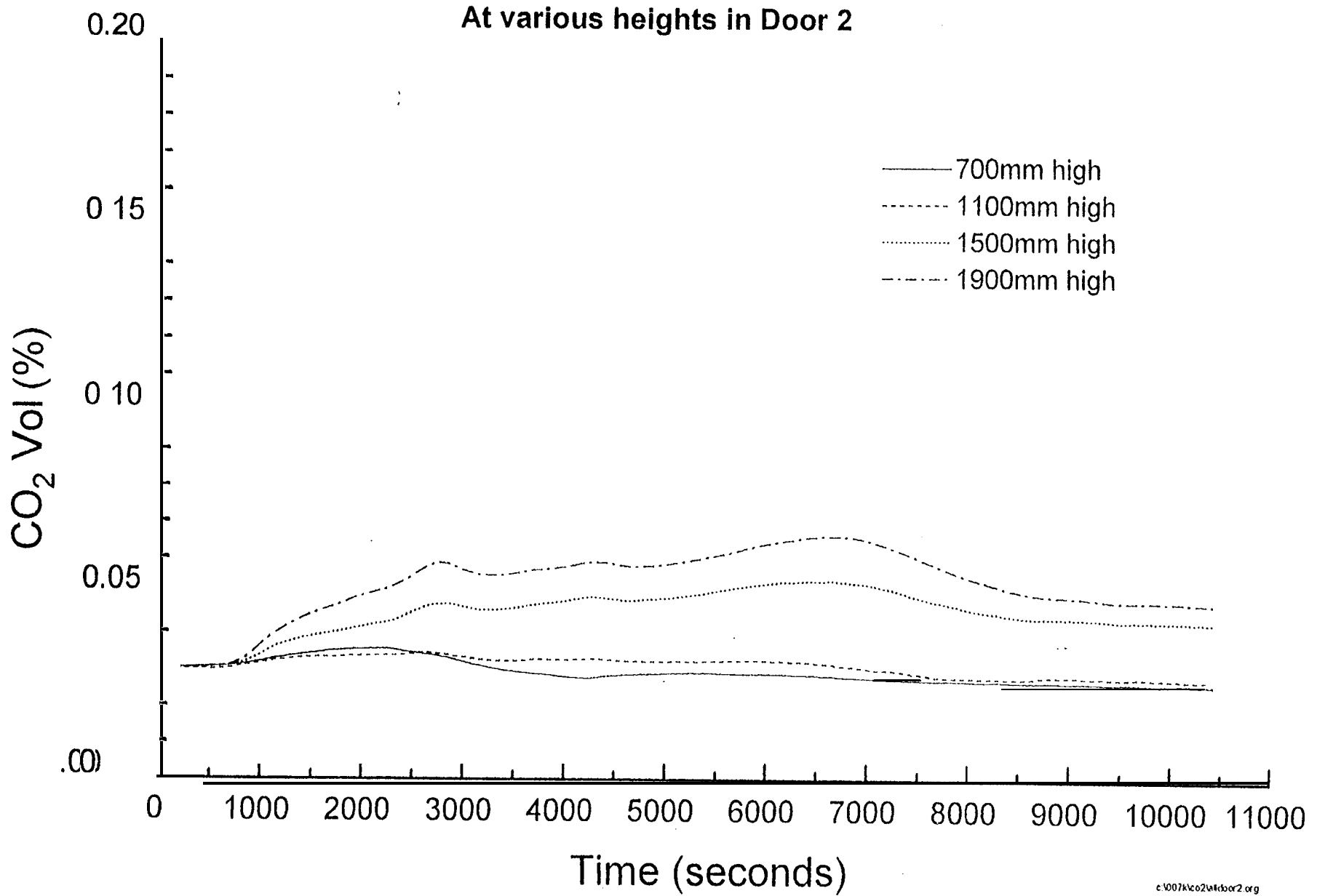
Fig. 6.2.5-7 Carbon dioxide concentration (Smouldering) - Test SM8
