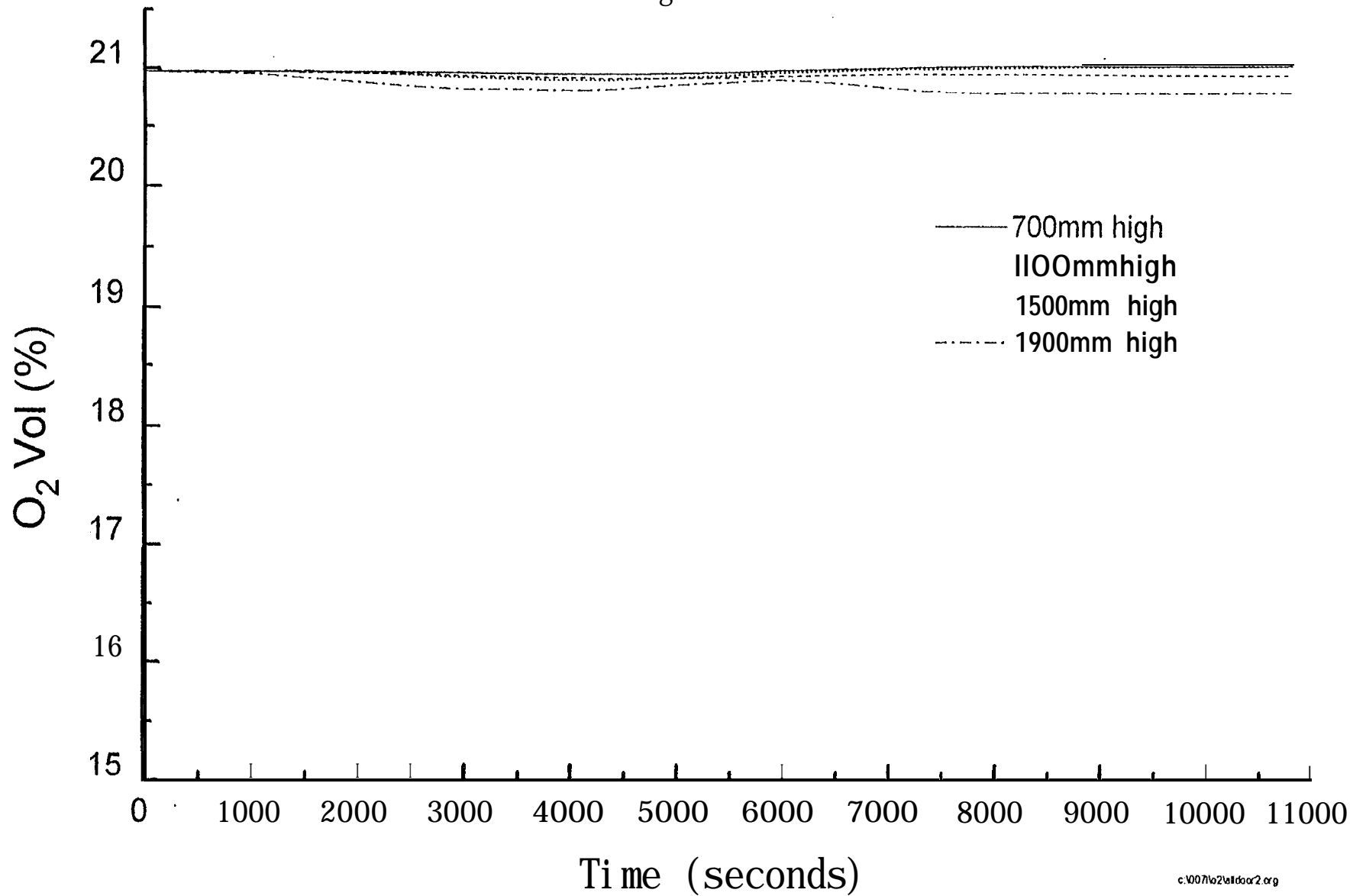
Fig. 6.2.4-7 Oxygen concentration (Smouldering) - Test SM7
