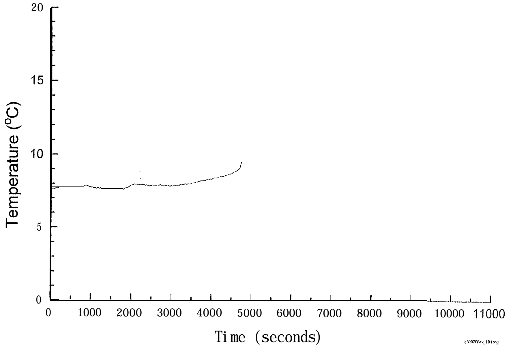
Average temperature in room 101 (Smouldering) - Test SM3
