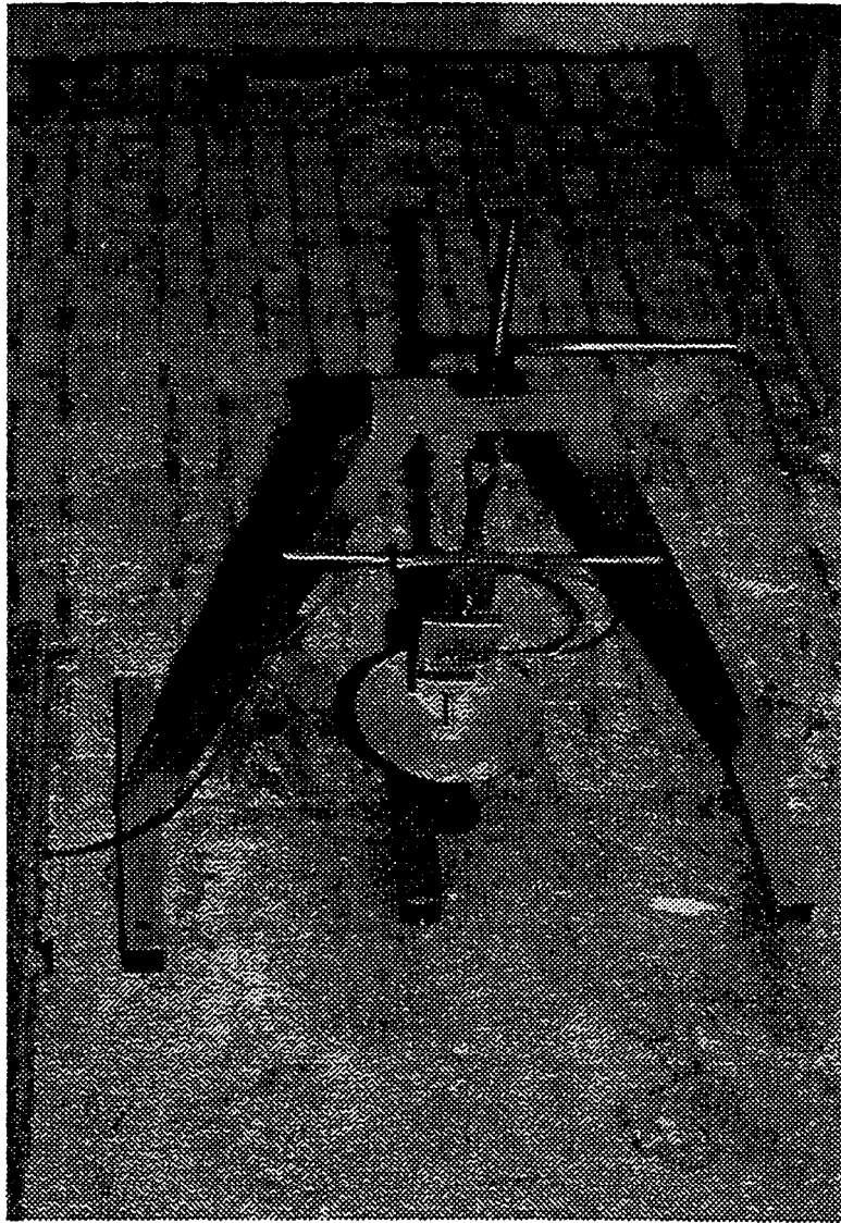
Figure A.10 Weighing system load cells and support assembly.
