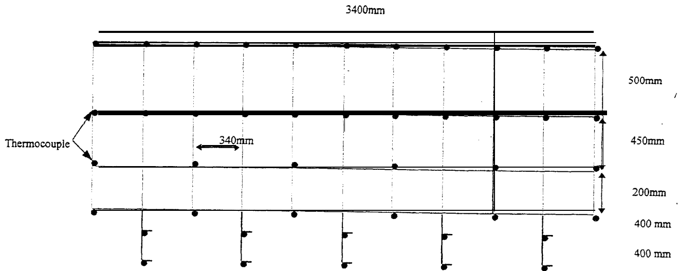
Figure 4-6 Thermocouple Rack T/C07 for Room 102
