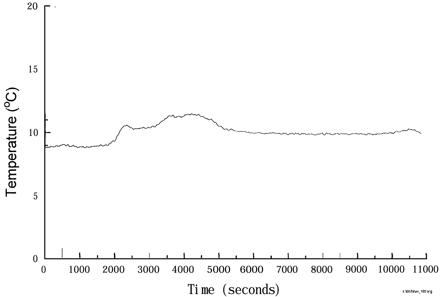
Fig. 6.2.2-7 Average temperature in room 102 (Smouldering) - Test SM7
