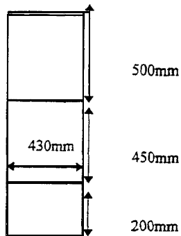
Figure 4-7 Thermocouple Rack T/C 08 for Room 102
