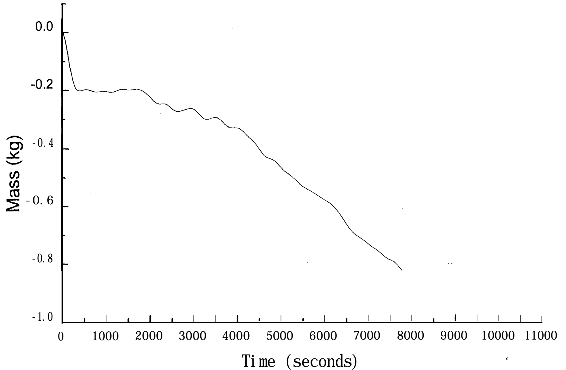
Mass loss (smouldering) - Test SM5
