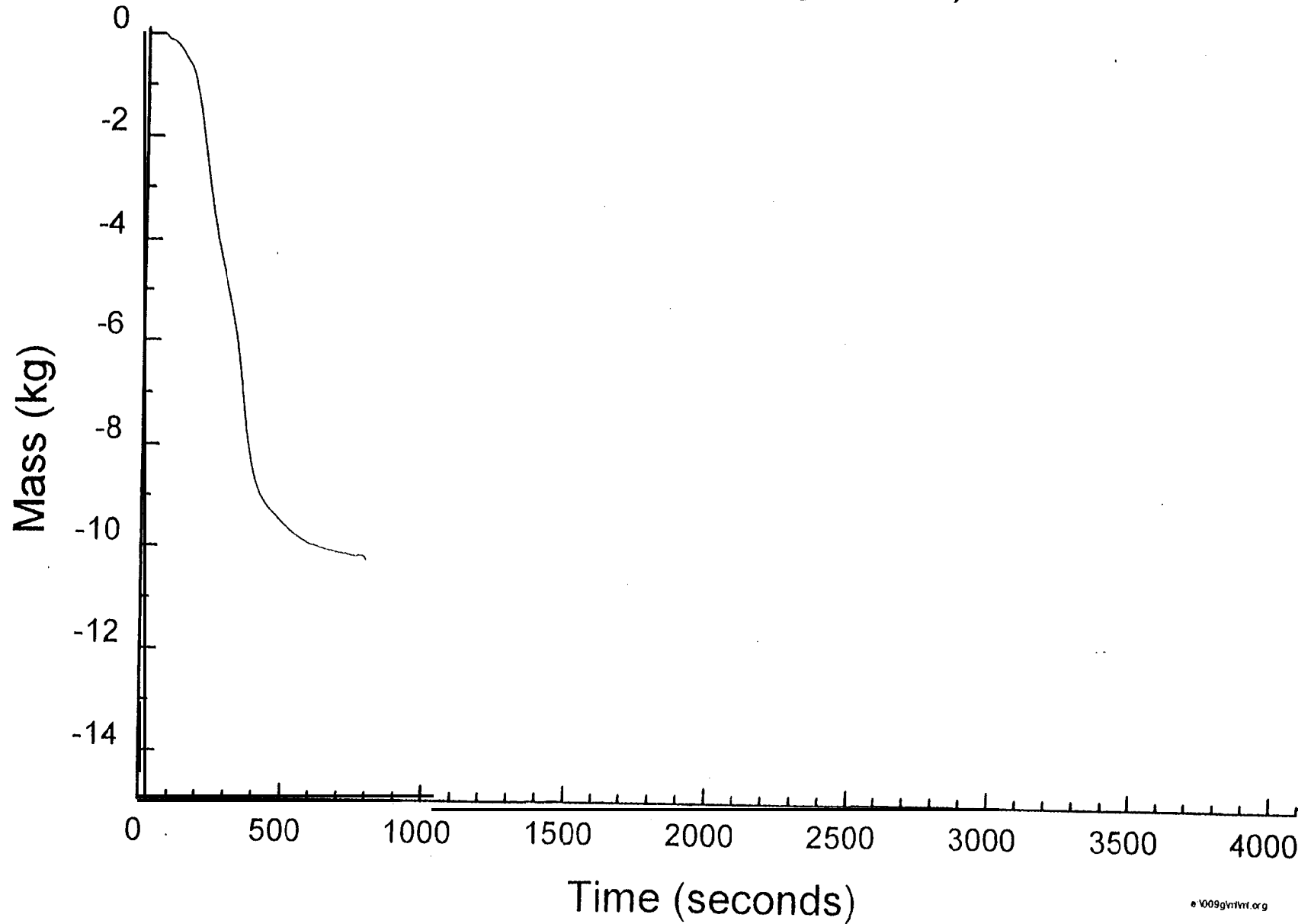
Mass loss (Flaming fire in large room) - Test FML6
