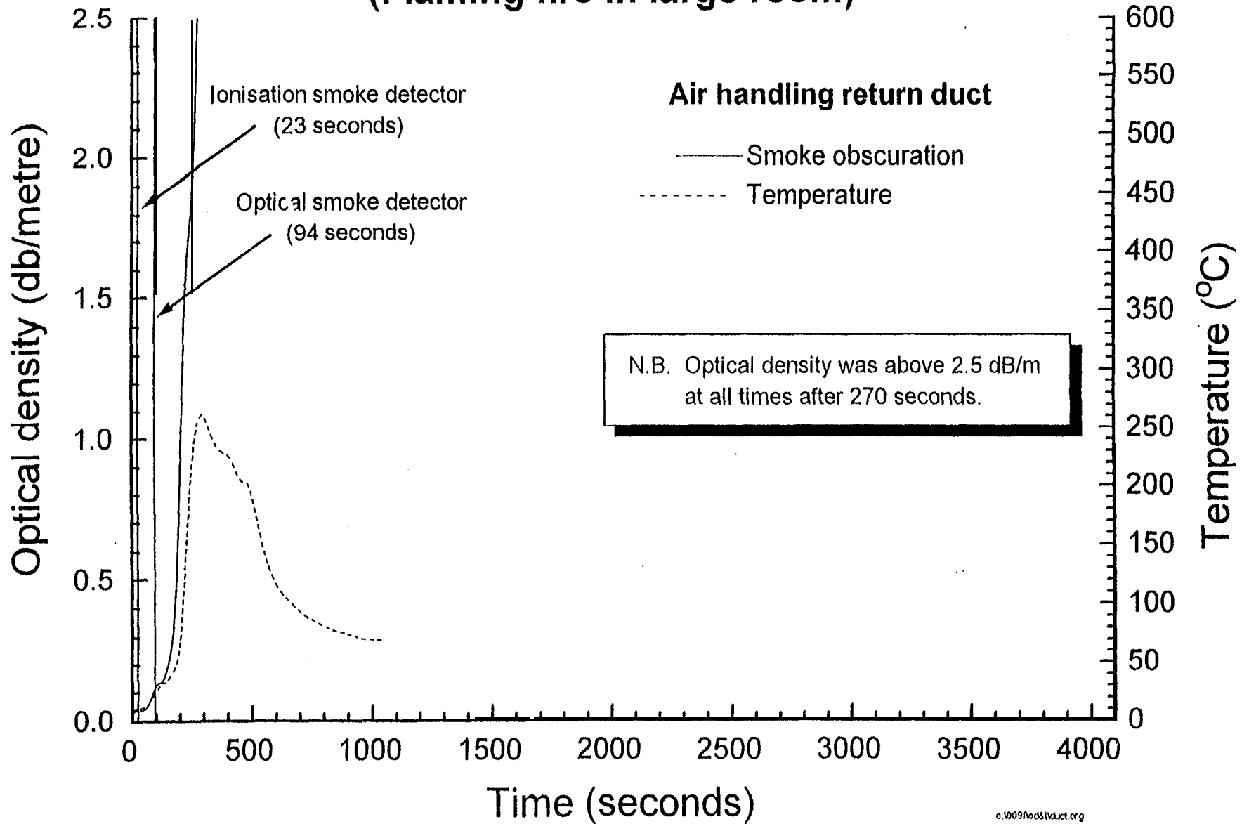
Fig. 8.2.8-8 Smoke obscuration and temperature - Test FML4 (Flaming fire in large room)
