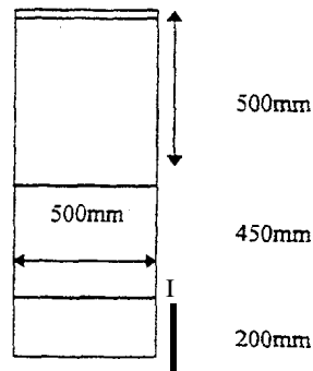
Figure 4-9 Thermocouple Rack T/C10 for Room 101
