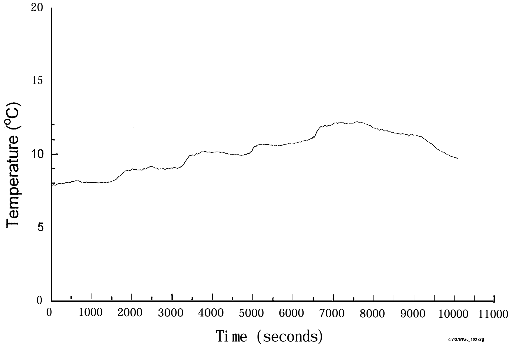
Fig. 6.2.2-2 Average temperature in room 102 (Smouldering) - Test SM2
