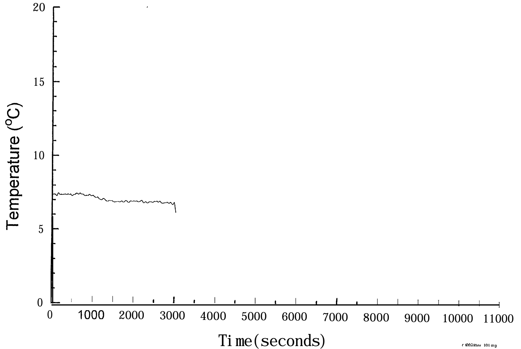
Fig. 6.2.2-I 2 Average temperature in room 101 (Smouldering) - Test SM4
