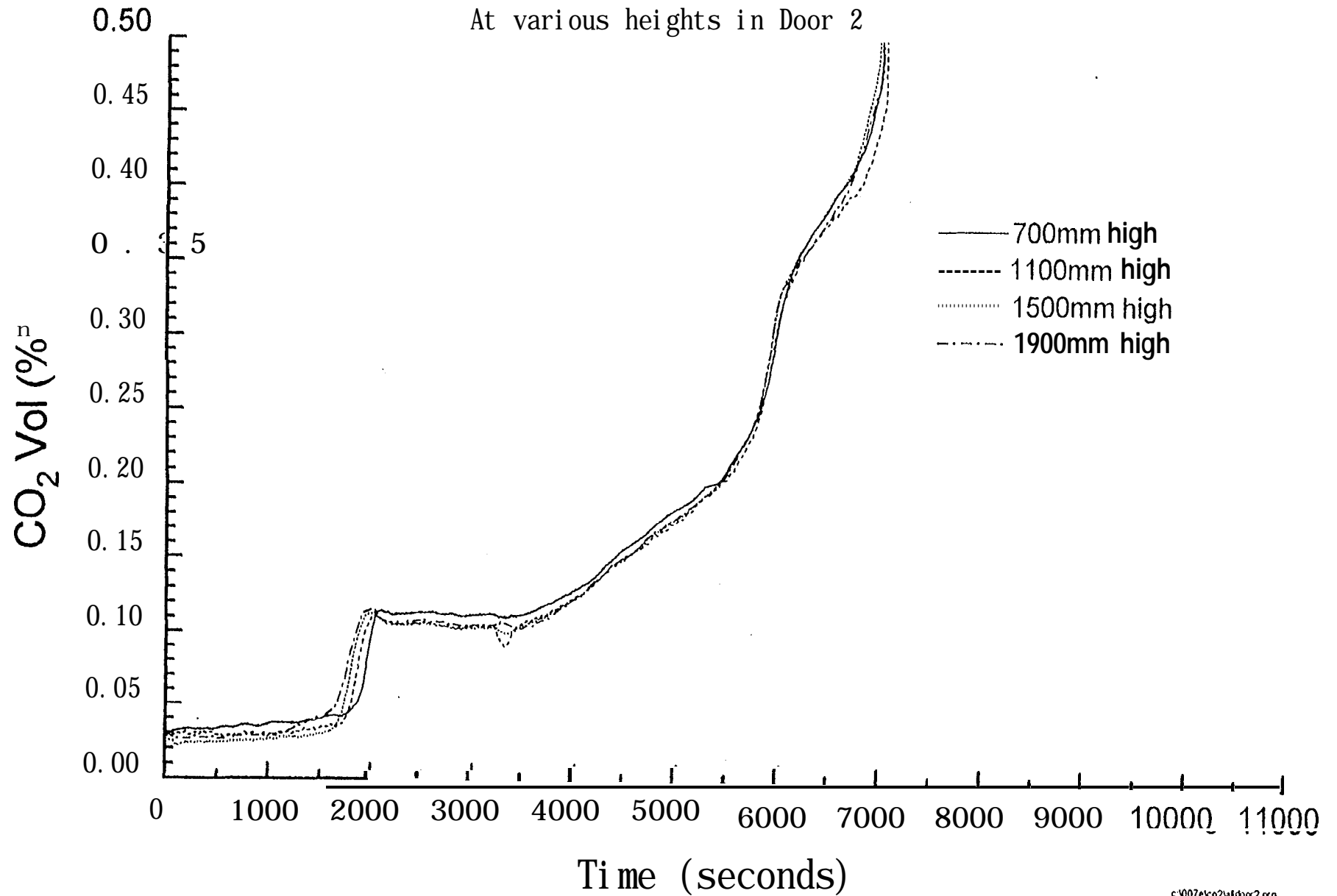
Fig. 6.251 Carbon dioxide concentration (Smouldering) - Test SM1
