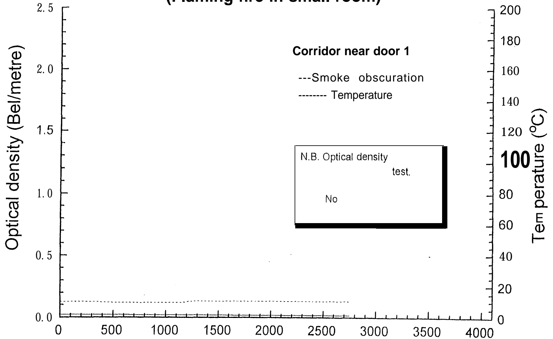
Fig. 7.3.7-8 Smoke obscuration and temperature - Test FMS5 (Flaming fire in small room)
