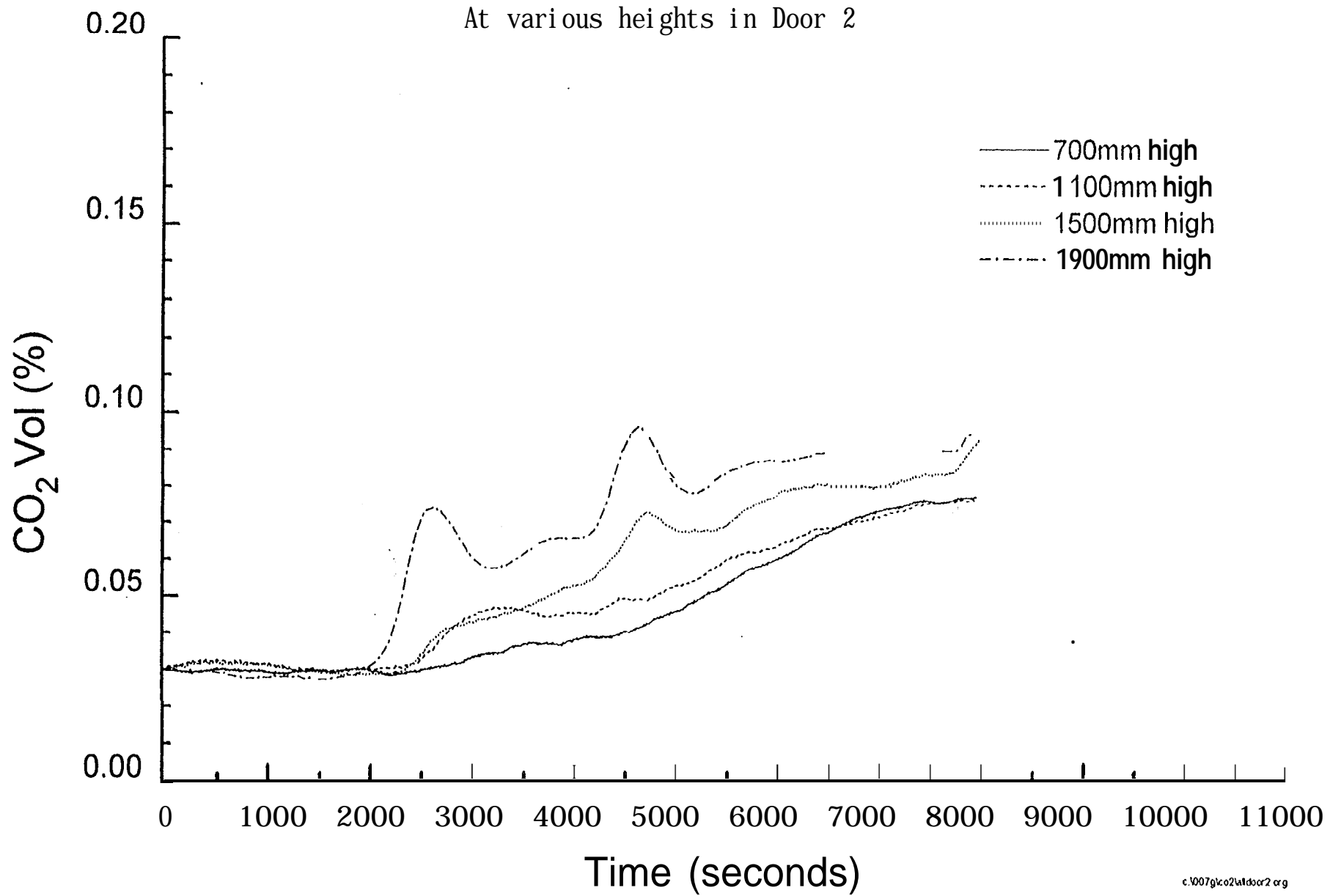
Fig. 6.2.5-4 Carbon dioxide concentration (Smouldering) - Test SM5
