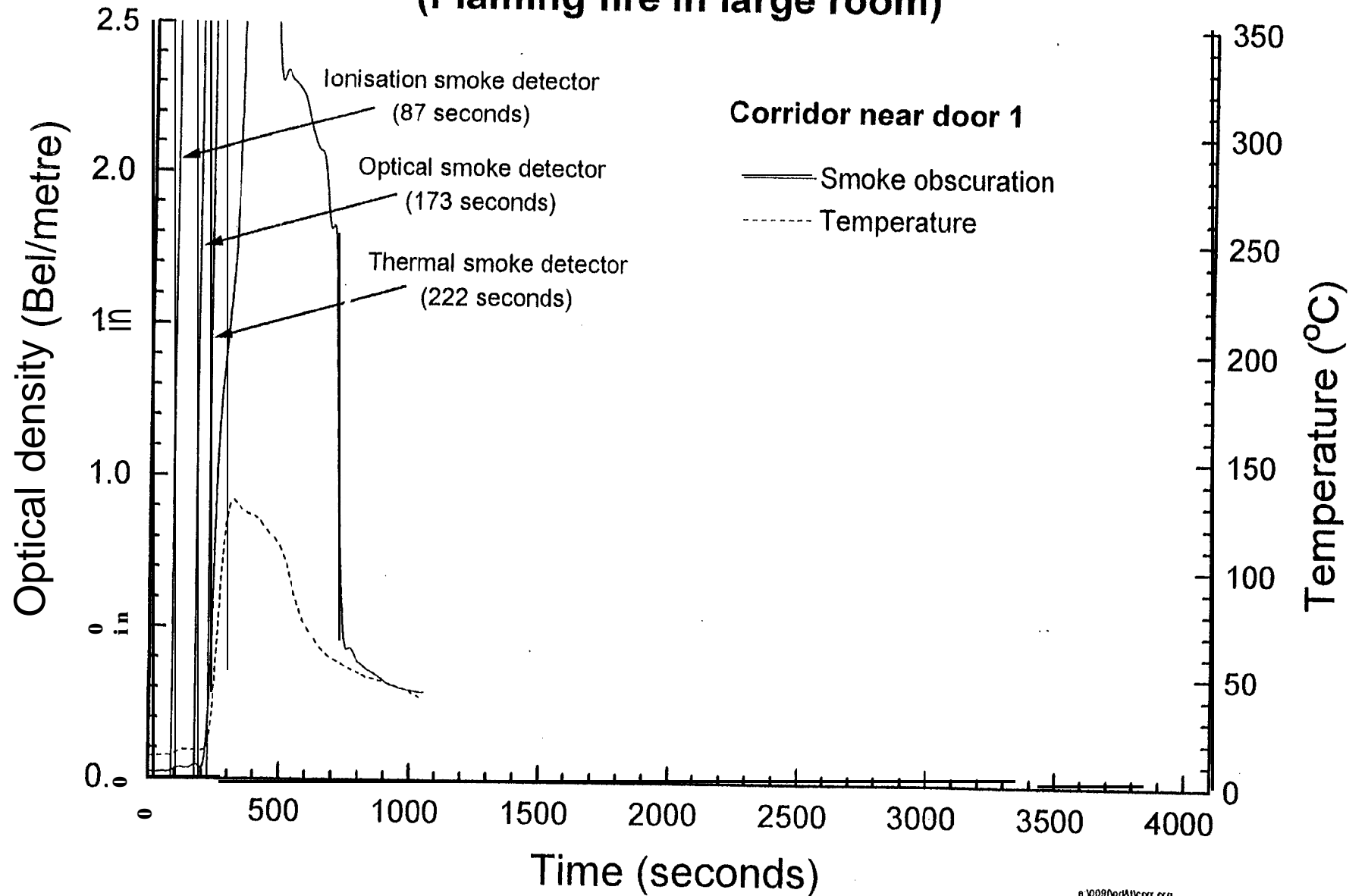
Fig. 8.2.8-4 Smoke obscuration and temperature - Test FM .4 (Flaming fire in large room)
