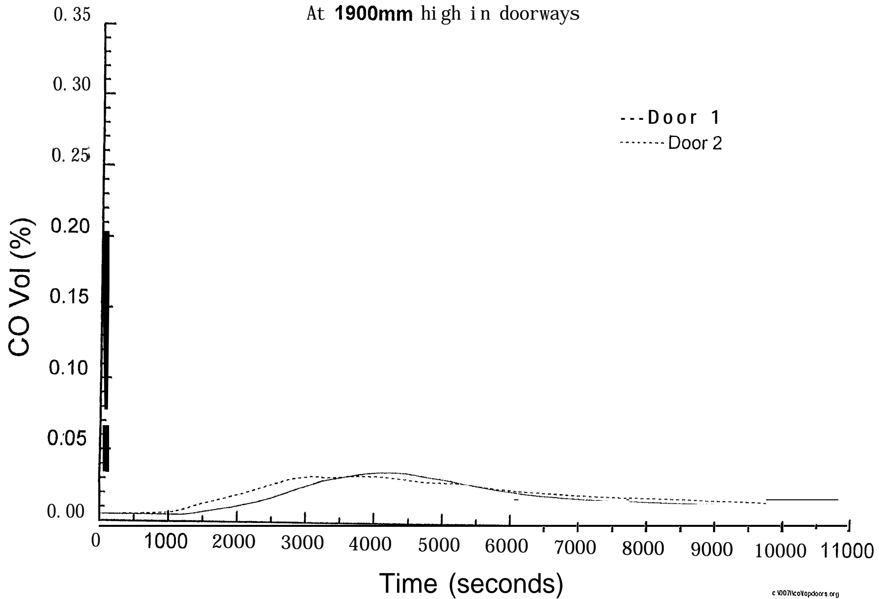
Fig. 6.2.3-7 Carbon monoxide concentration (Smouldering) - Test SM7
