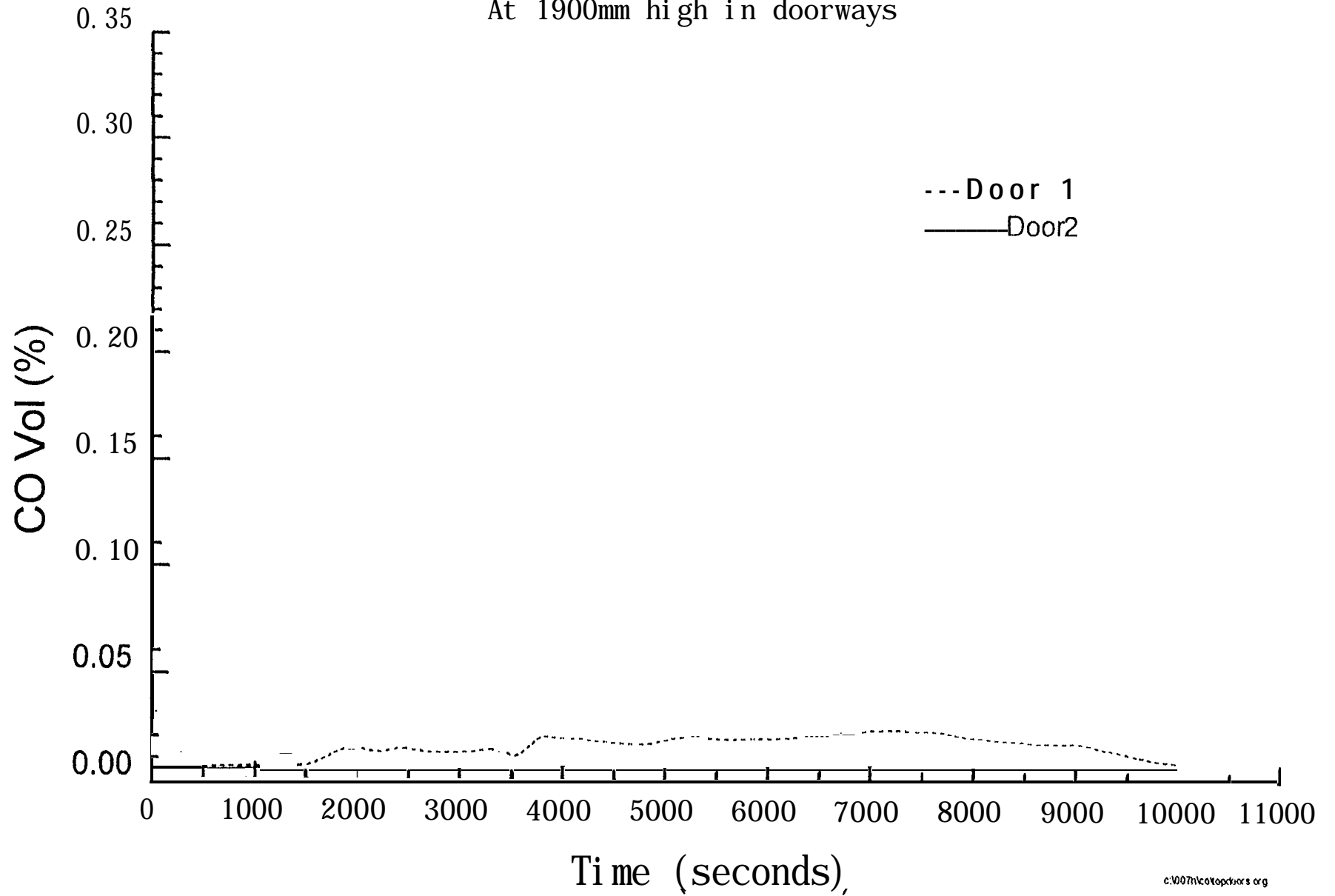
Fig. 6.2.3-2 Carbon monoxide concentration (Smouldering) - Test SM2
