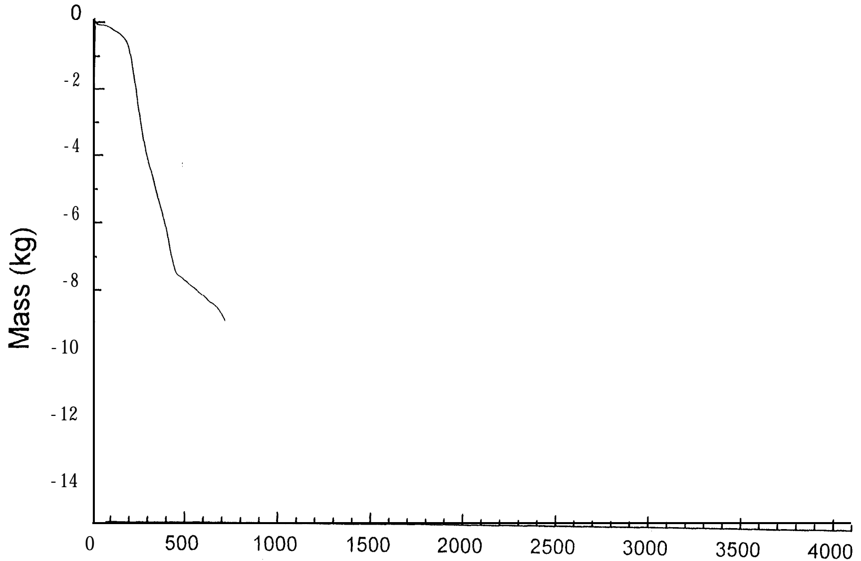
Mass loss (Flaming fire in large room) - Test FML2
