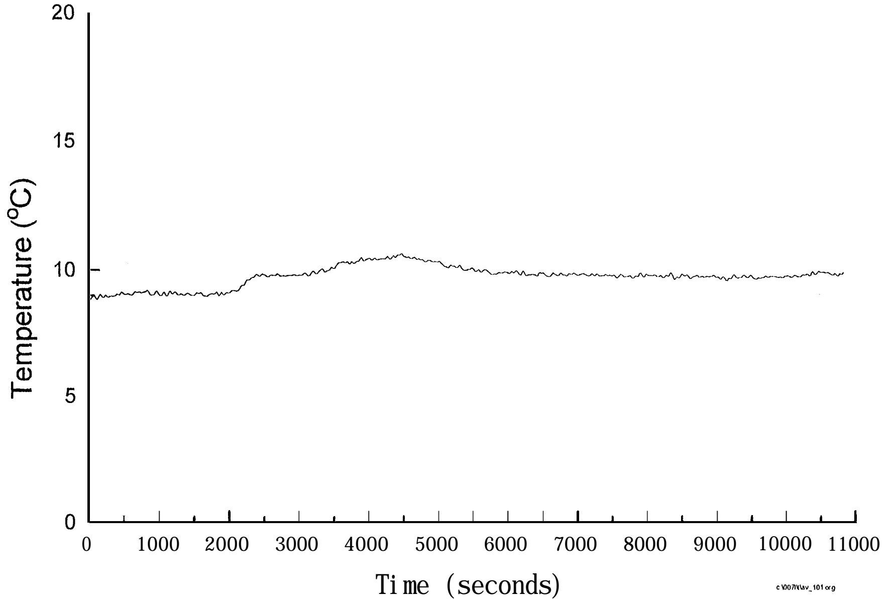
Average temperature in room 101 (Smouldering) - Test SM7
