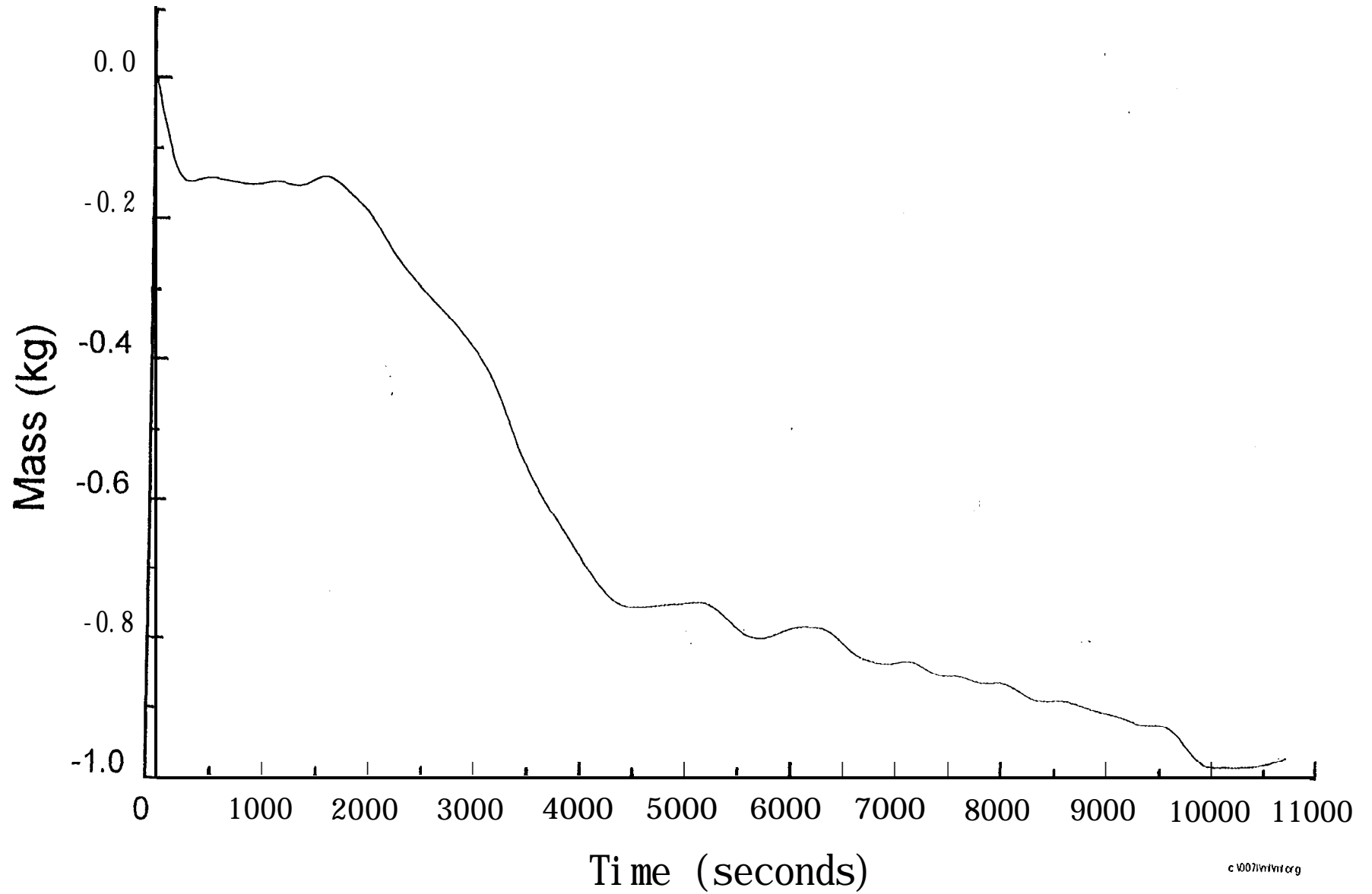
Fig. 6.2.1-7 Mass loss (smouldering) - Test SM7
