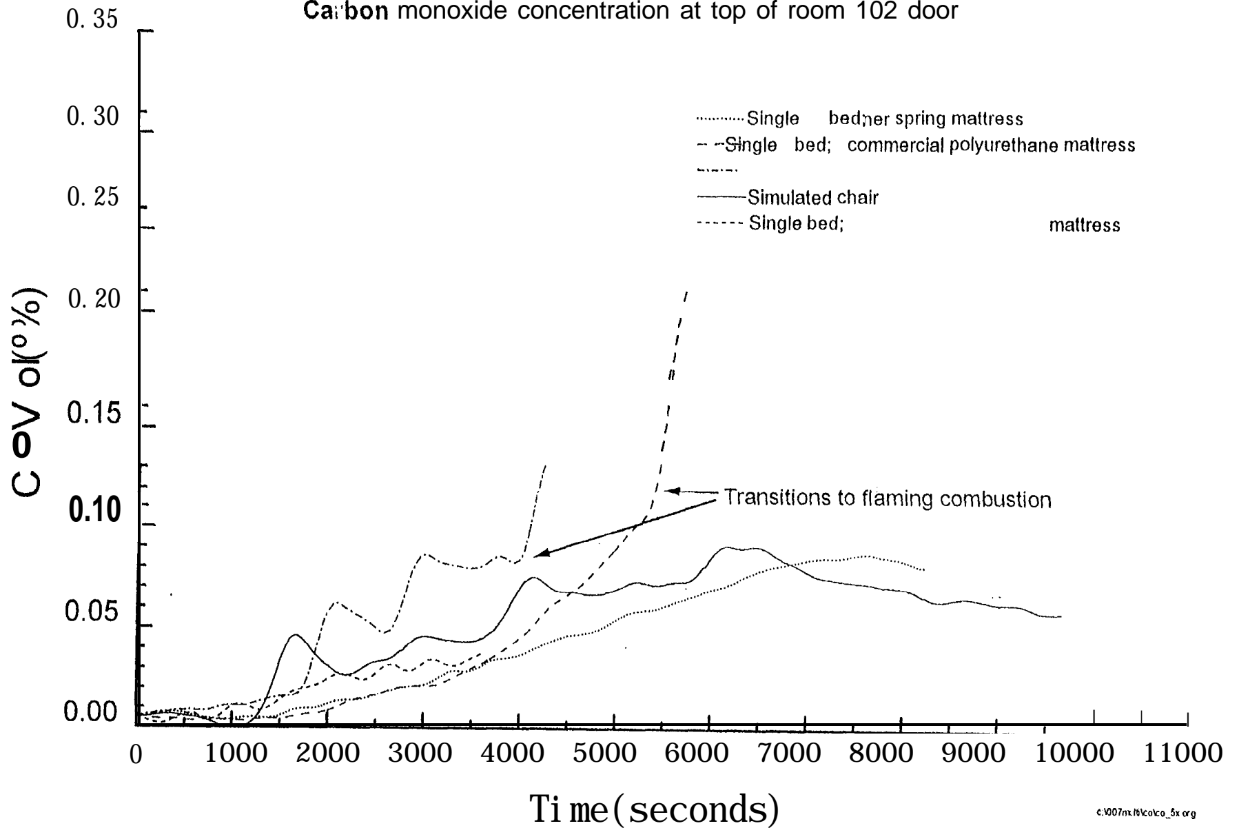
Fig. 6.1.2-1 Commercial product tests (smouldering)
