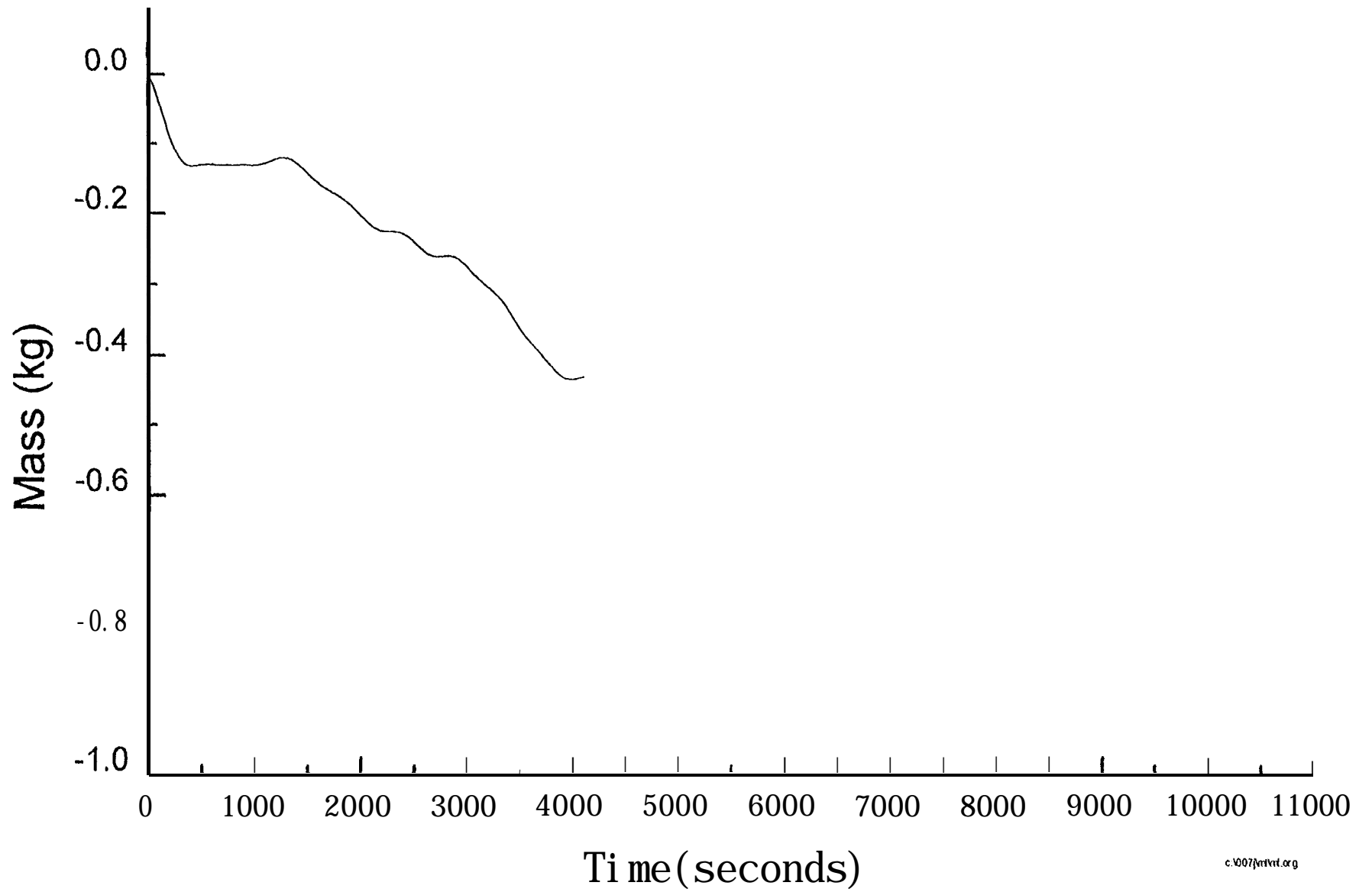
Fig. 6.2.1-6 Mass loss (smouldering) - Test SM6
