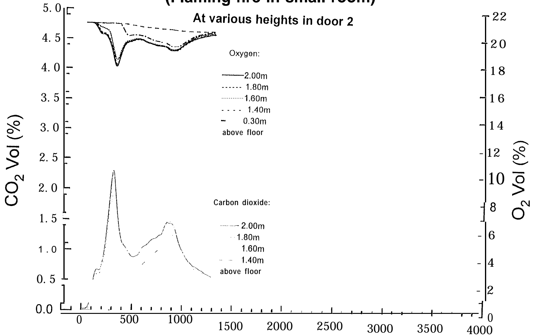
Fig. 7.3.6-I 2 Carbon dioxide and Oxygen concentrations - Test FMS10 (Flaming fire in small room)
