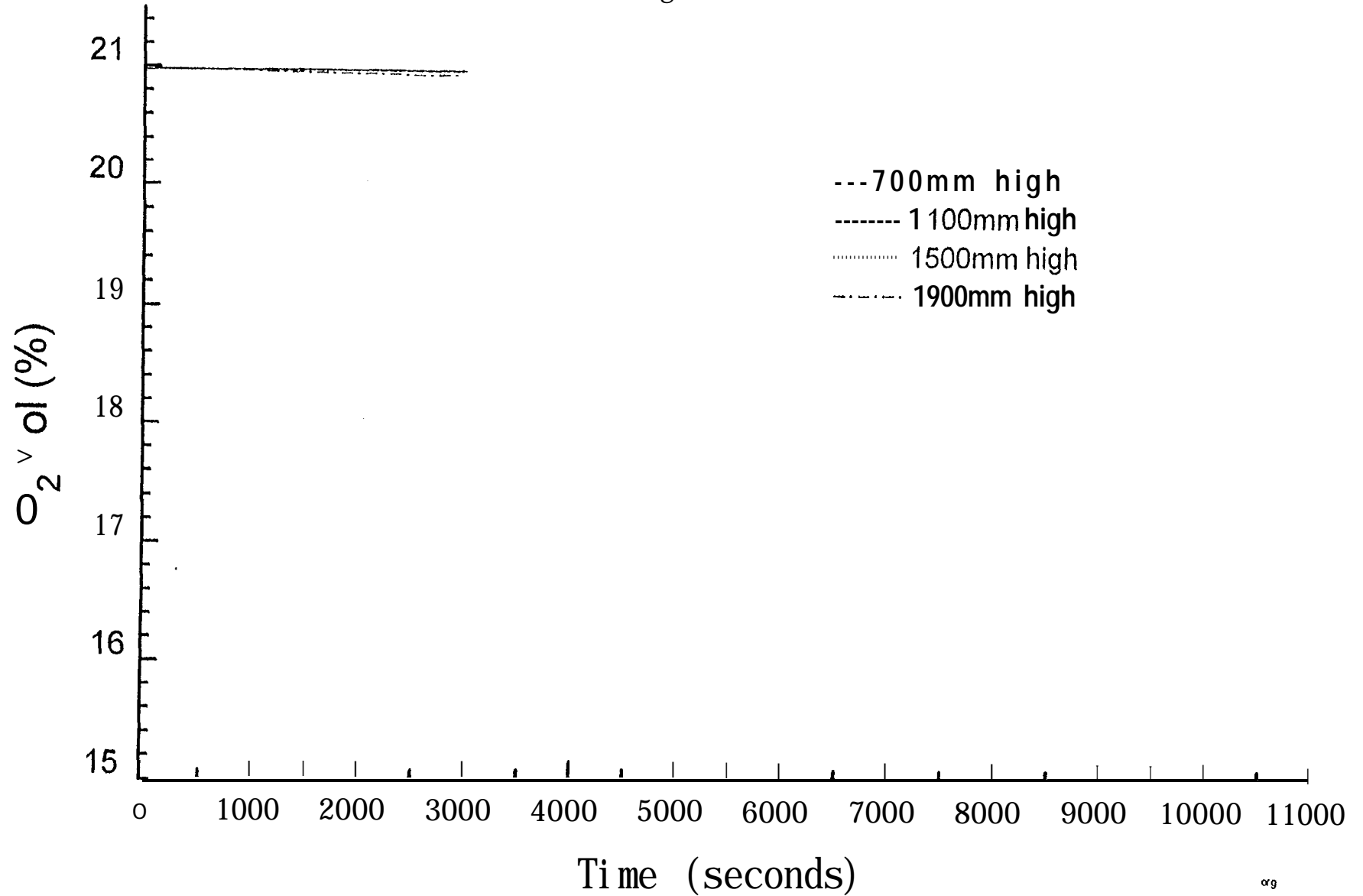
Fig. 6.2.4-4 Oxygen concentration (Smouldering) - Test SM4
