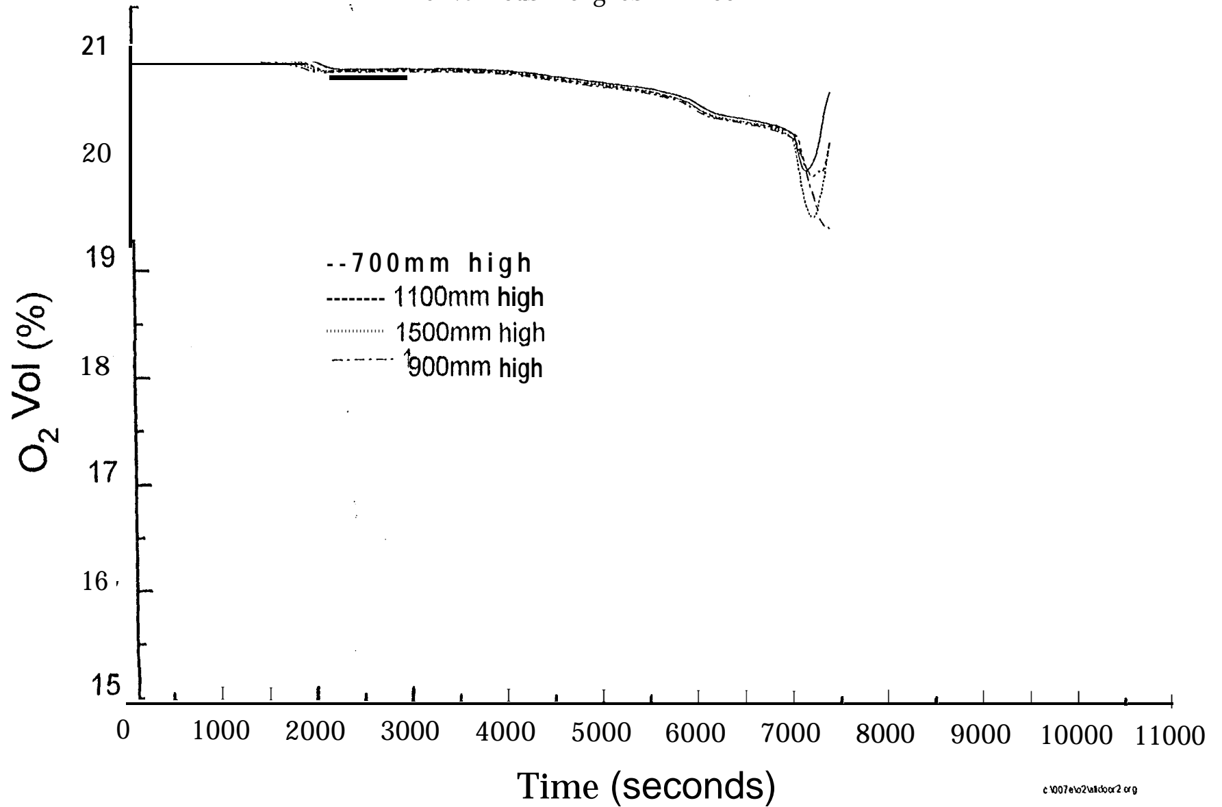
Fig. 6.2.4-I Oxygen concentration (Smouldering) - Test SM1
