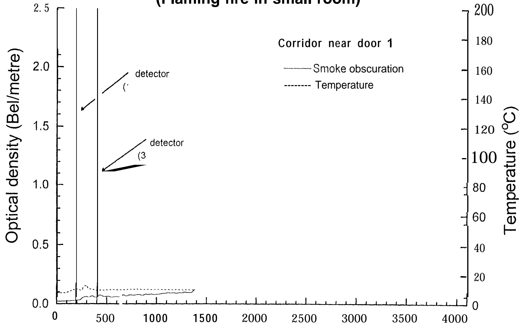
Fig. 7.3.7-9 Smoke obscuration and temperature - Test FMS6 (Flaming fire in small room)
