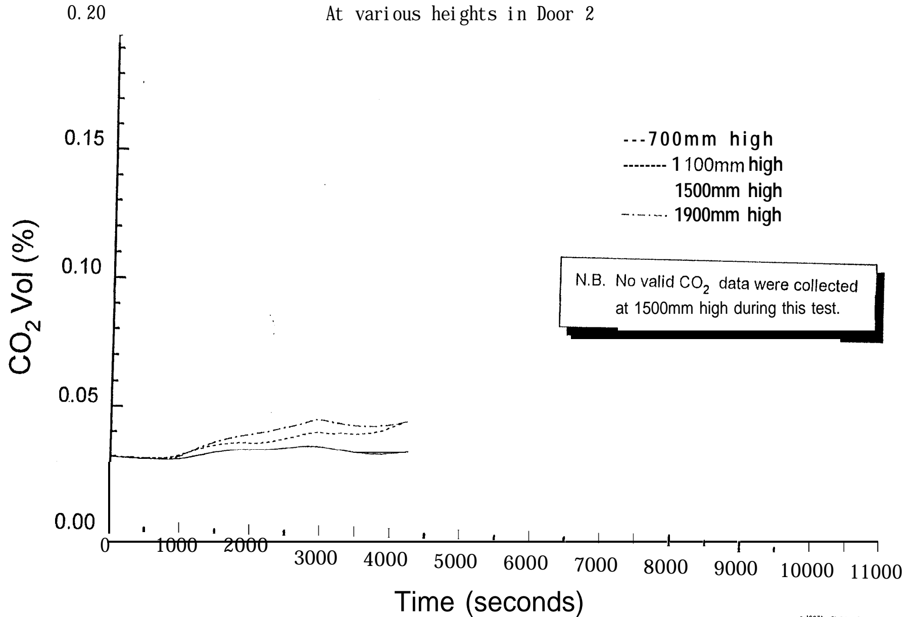
Fig. 6.2.5-5 Carbon dioxide concentration (Smouldering) - Test SM6
