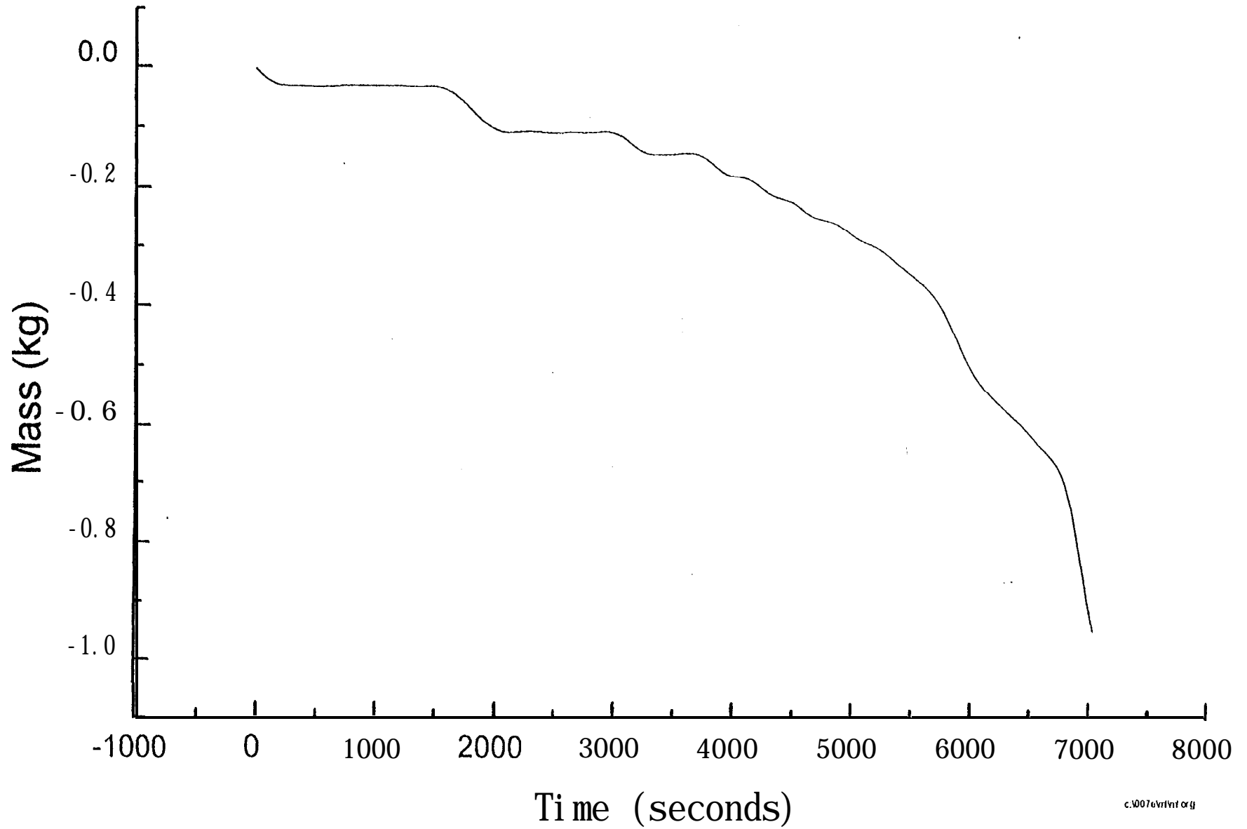
Fig. 6.2.1-I Mass loss (smouldering) - Test SM1
