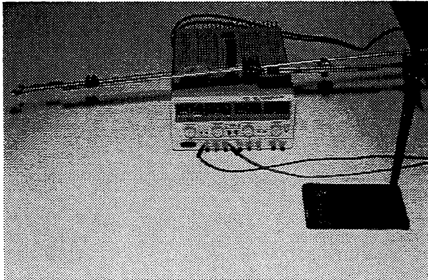
Figure A.1 Electric igniter
