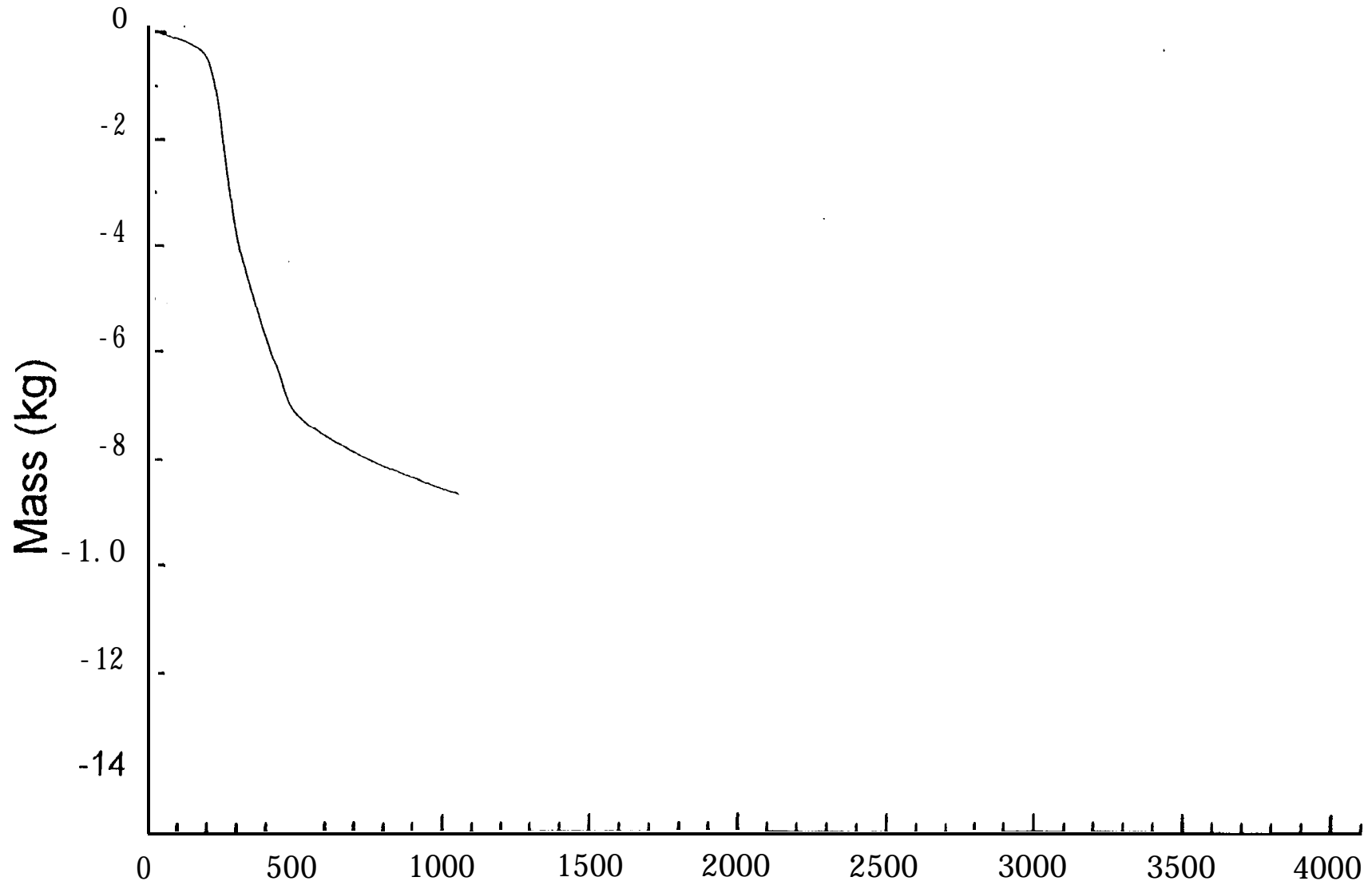
Mass loss (Flaming fire in large room) - Test FML4
