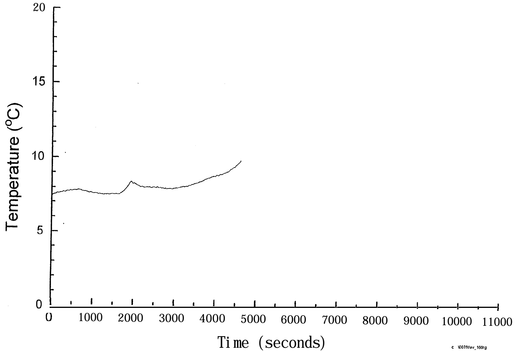
Fig. 6.2.2-3 Average temperature in room 102 (Smouldering) - Test SM3
