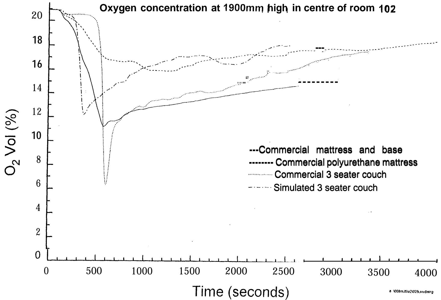
Fig. 8.1.3-I Commercial product tests (Flaming fire in large room)
