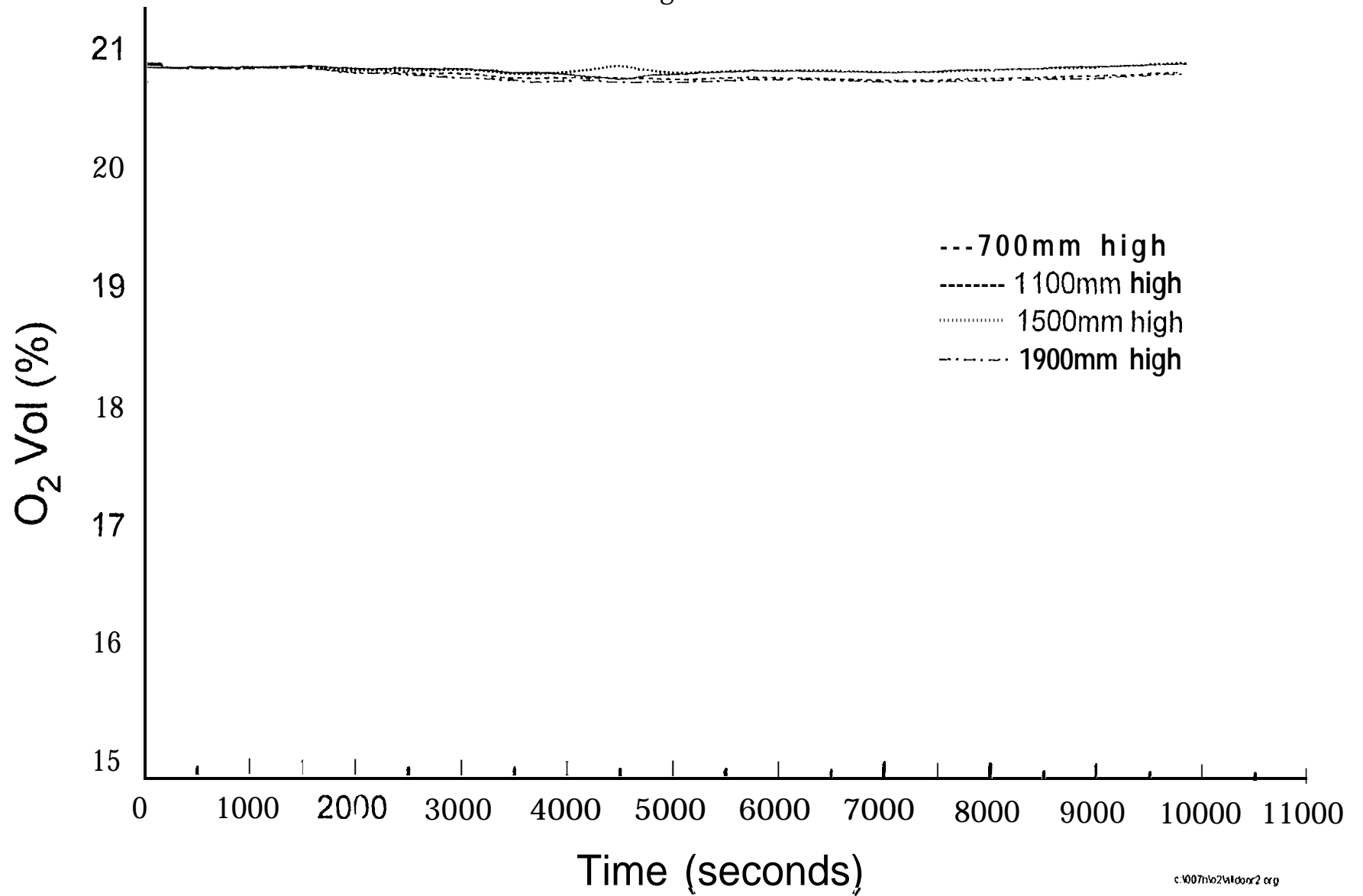
Fig. 6.2.4-2 Oxygen concentration (Smouldering) - Test SM2
