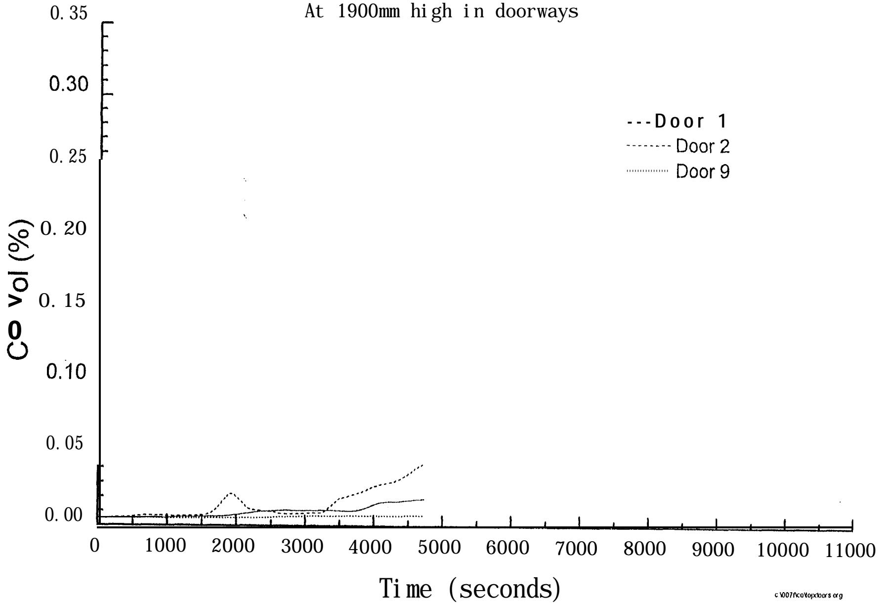
Fig. 6.2.3-3 Carbon' monoxide concentration (Smouldering) - Test SM3
