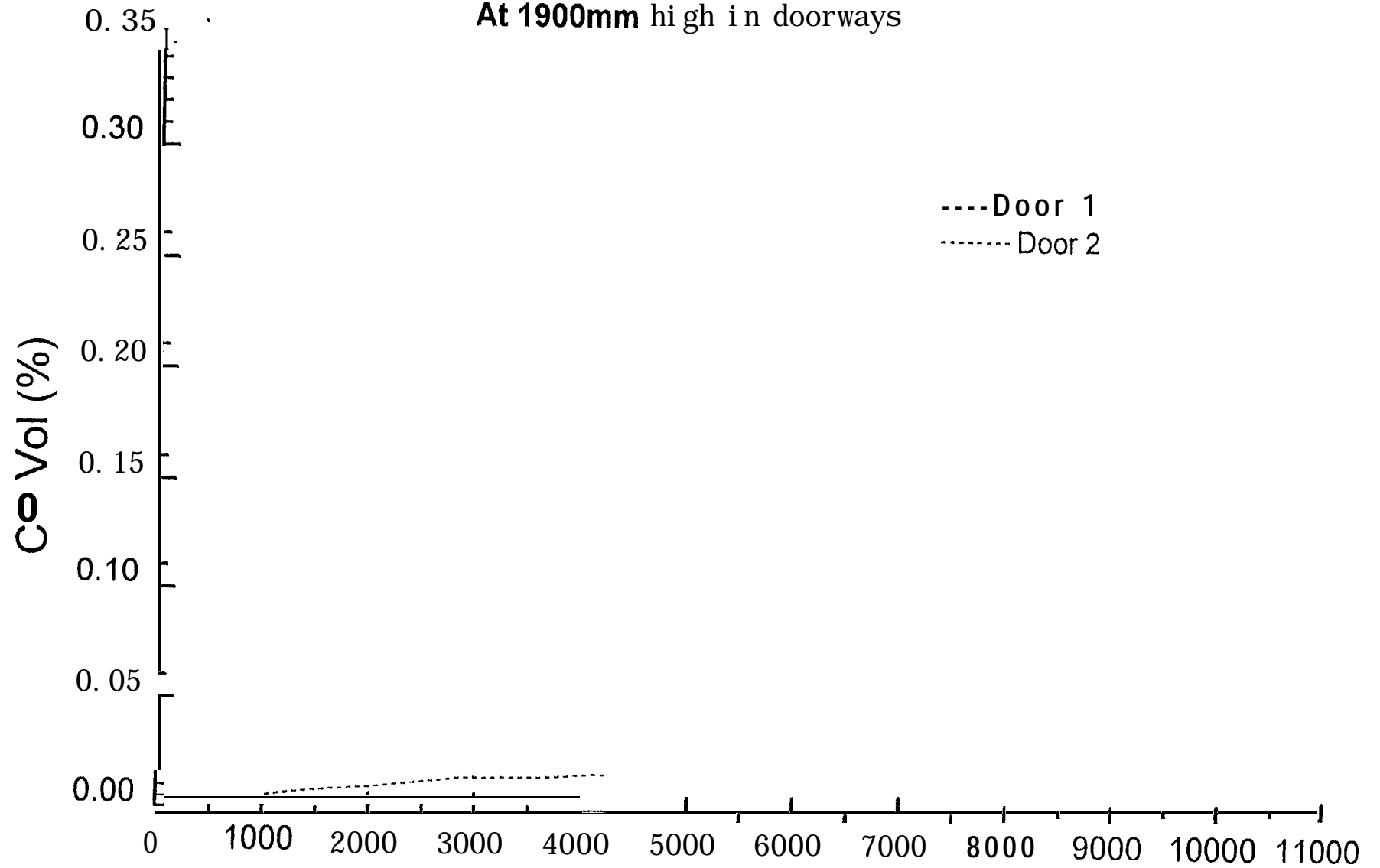
Fig. 6.2.3-6 Carbon monoxide concentration (Smouldering) - Test SM6
