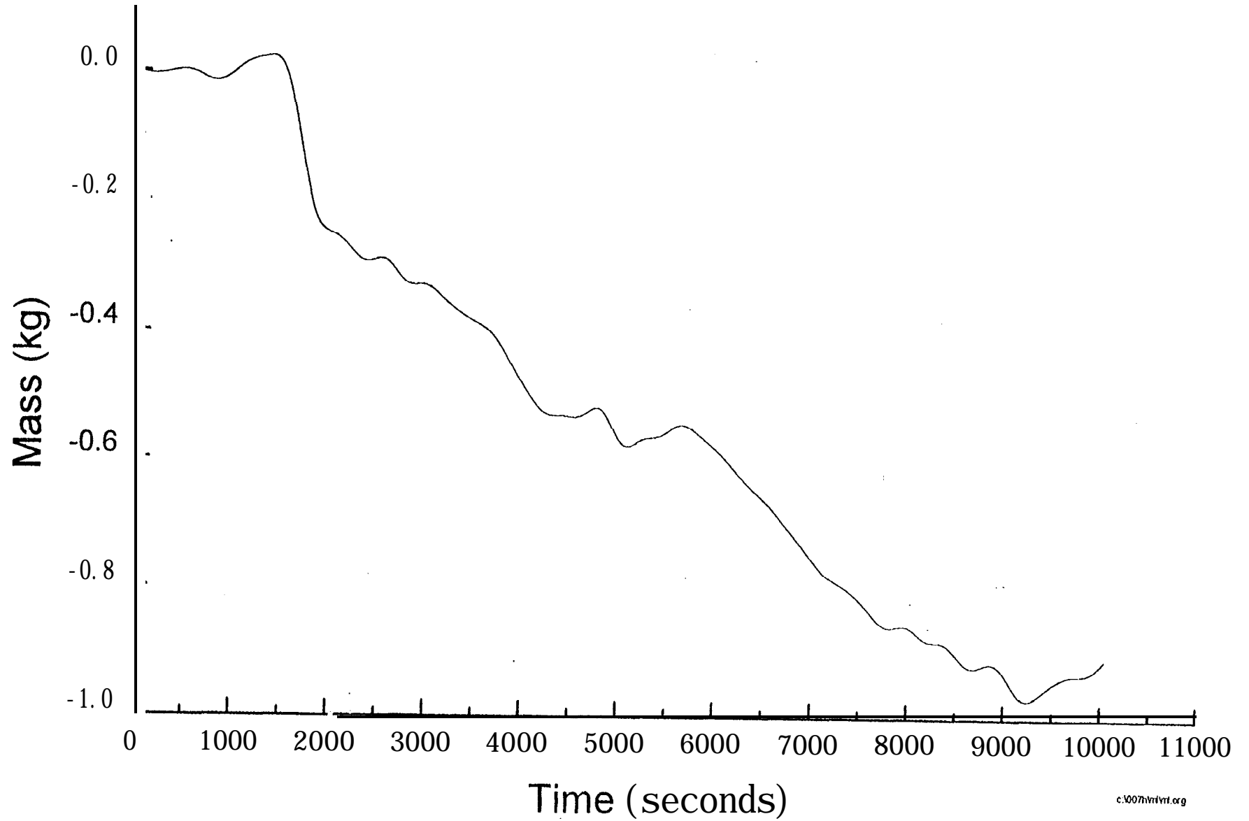
Fig. 6.2.1-2 Mass loss (smouldering) - Test SM2
