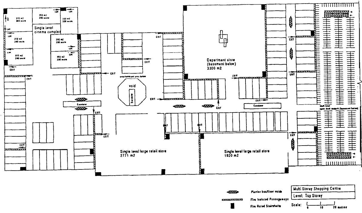
FIGURE 8.1 GENERALISED LAYOUT FOR A DOUBLE STOREY SHOPPING CENTRE, TO BE USED FOR RISK ASSESSMENT MODELLING
